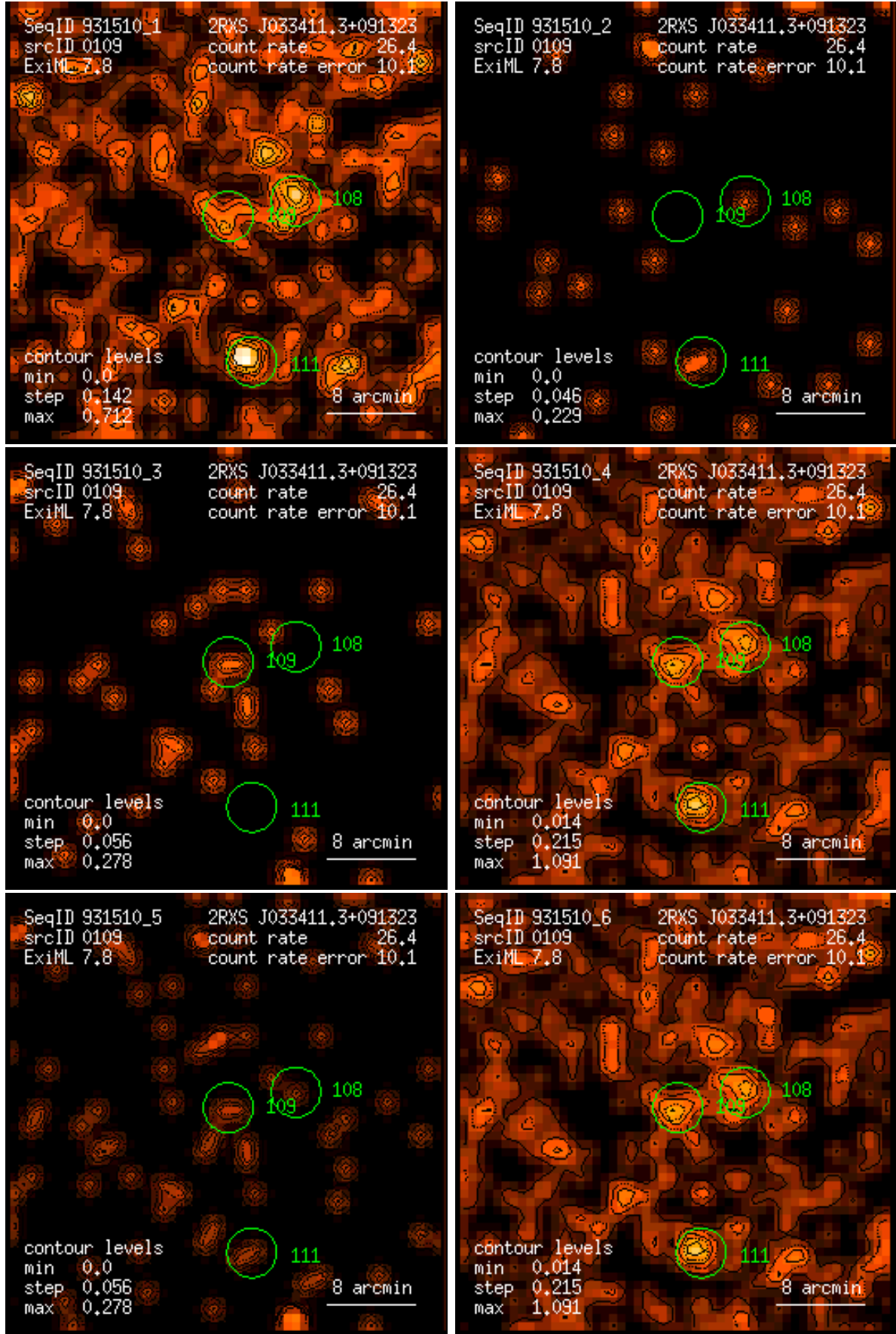
Figure 109: RASS 931510: detection 0109: band rate images, Gaussian filter: (1) PSPC channels 11 – 41, (2) 52 – 90, (3) 91 – 201, (4) 11 – 235, (5) 52 – 201, (6) 11 – 201. Broad band rates in counts/ks. Band rate contour levels in counts/ks/arcmin 2 .
