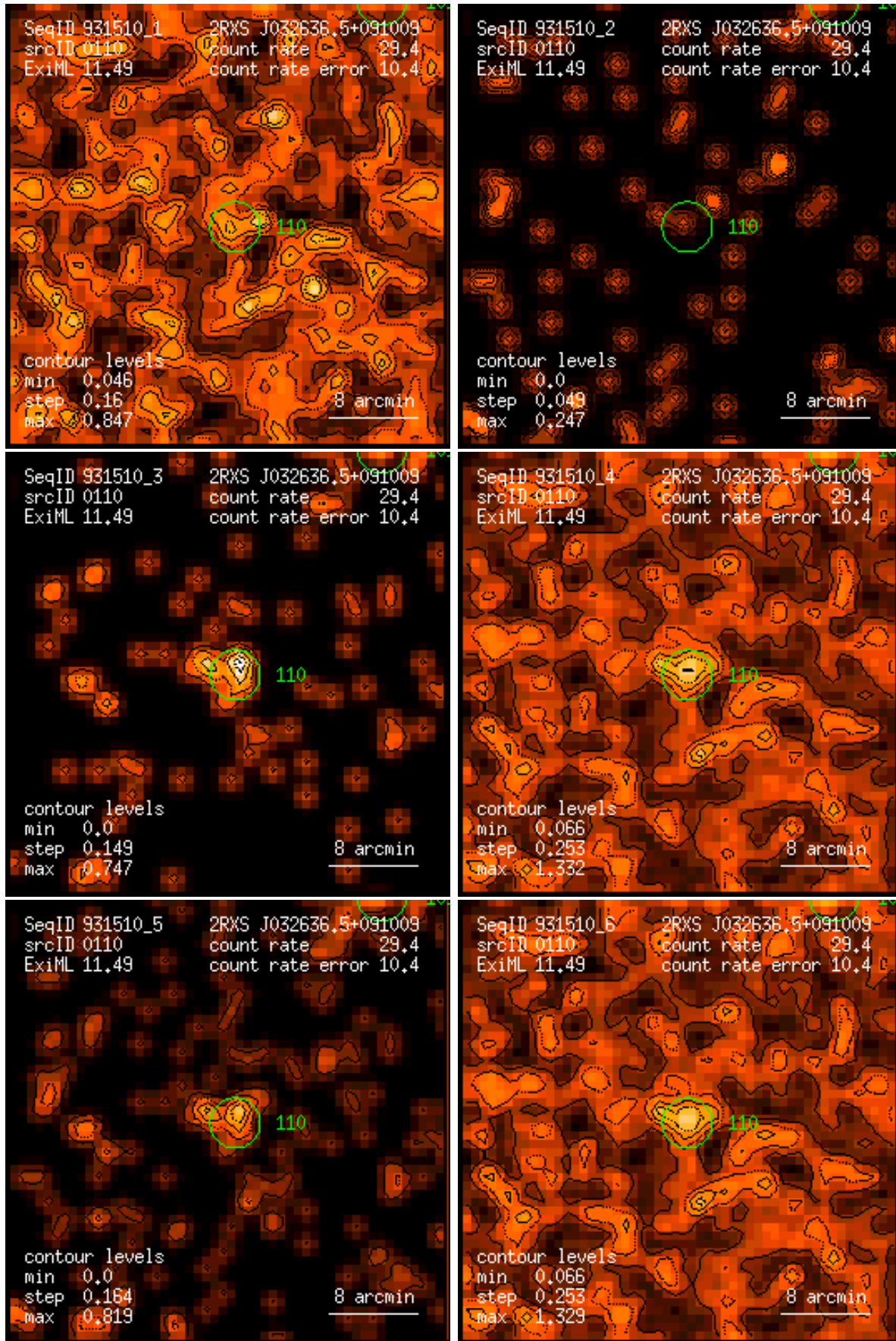
Figure 110: RASS 931510: detection 0110: band rate images, Gaussian filter: (1) PSPC channels 11 – 41, (2) 52 – 90, (3) 91 – 201, (4) 11 – 235, (5) 52 – 201, (6) 11 – 201. Broad band rates in counts/ks. Band rate contour levels in counts/ks/arcmin 2 .
