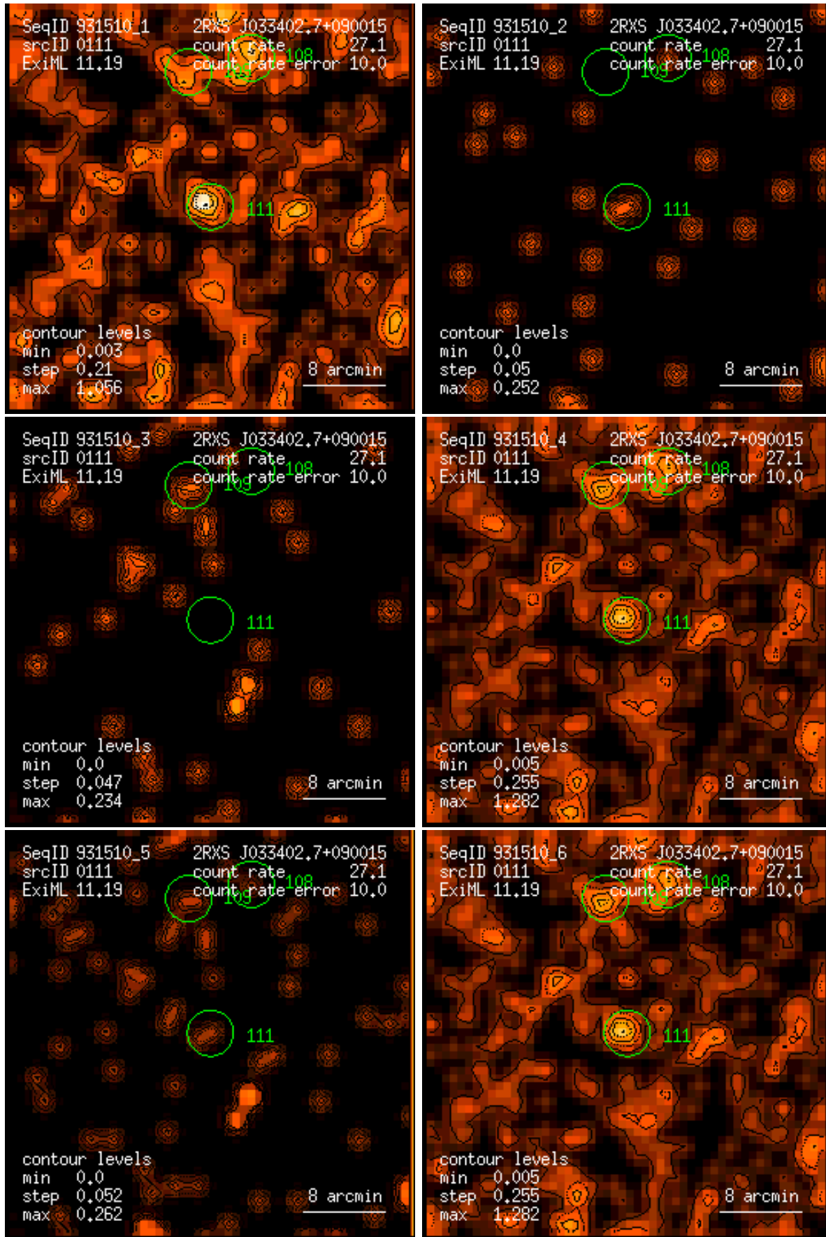
Figure 111: RASS 931510: detection 0111: band rate images, Gaussian filter: (1) PSPC channels 11 – 41, (2) 52 – 90, (3) 91 – 201, (4) 11 – 235, (5) 52 – 201, (6) 11 – 201. Broad band rates in counts/ks. Band rate contour levels in counts/ks/arcmin 2 .
