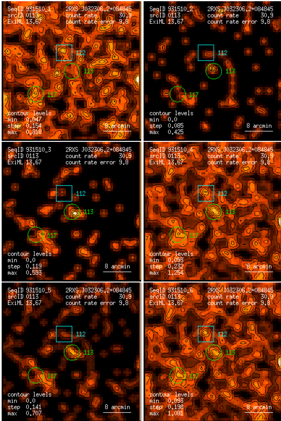
Figure 113: RASS 931510: detection 0113: band rate images, Gaussian filter: (1) PSPC channels 11 – 41, (2) 52 – 90, (3) 91 – 201, (4) 11 – 235, (5) 52 – 201, (6) 11 – 201. Broad band rates in counts/ks. Band rate contour levels in counts/ks/arcmin 2 .
