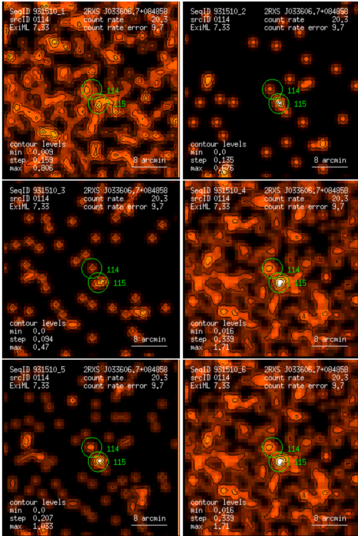
Figure 114: RASS 931510: detection 0114: band rate images, Gaussian filter: (1) PSPC channels 11 – 41, (2) 52 – 90, (3) 91 – 201, (4) 11 – 235, (5) 52 – 201, (6) 11 – 201. Broad band rates in counts/ks. Band rate contour levels in counts/ks/arcmin 2 .
