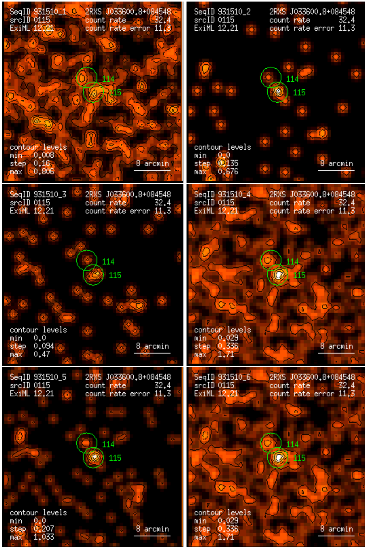
Figure 115: RASS 931510: detection 0115: band rate images, Gaussian filter: (1) PSPC channels 11 – 41, (2) 52 – 90, (3) 91 – 201, (4) 11 – 235, (5) 52 – 201, (6) 11 – 201. Broad band rates in counts/ks. Band rate contour levels in counts/ks/arcmin 2 .
