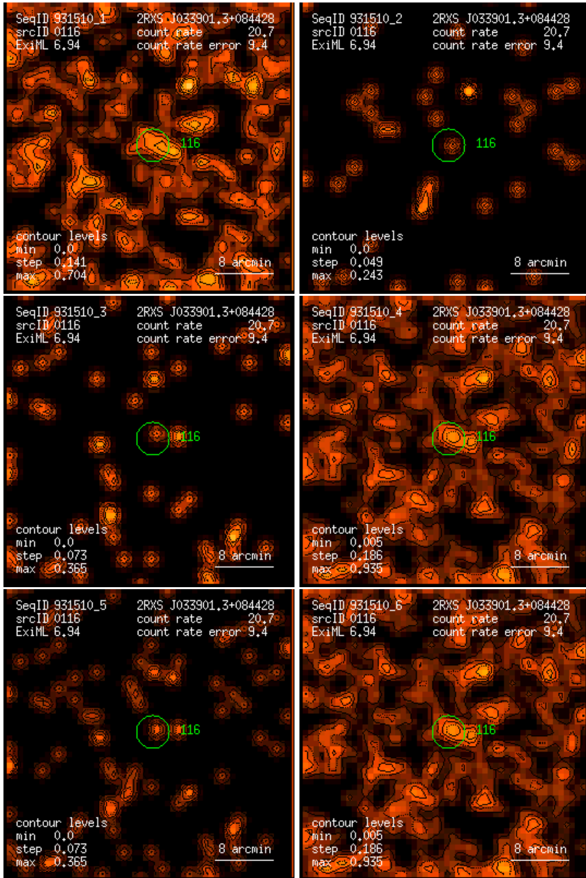
Figure 116: RASS 931510: detection 0116: band rate images, Gaussian filter: (1) PSPC channels 11 – 41, (2) 52 – 90, (3) 91 – 201, (4) 11 – 235, (5) 52 – 201, (6) 11 – 201. Broad band rates in counts/ks. Band rate contour levels in counts/ks/arcmin 2 .
