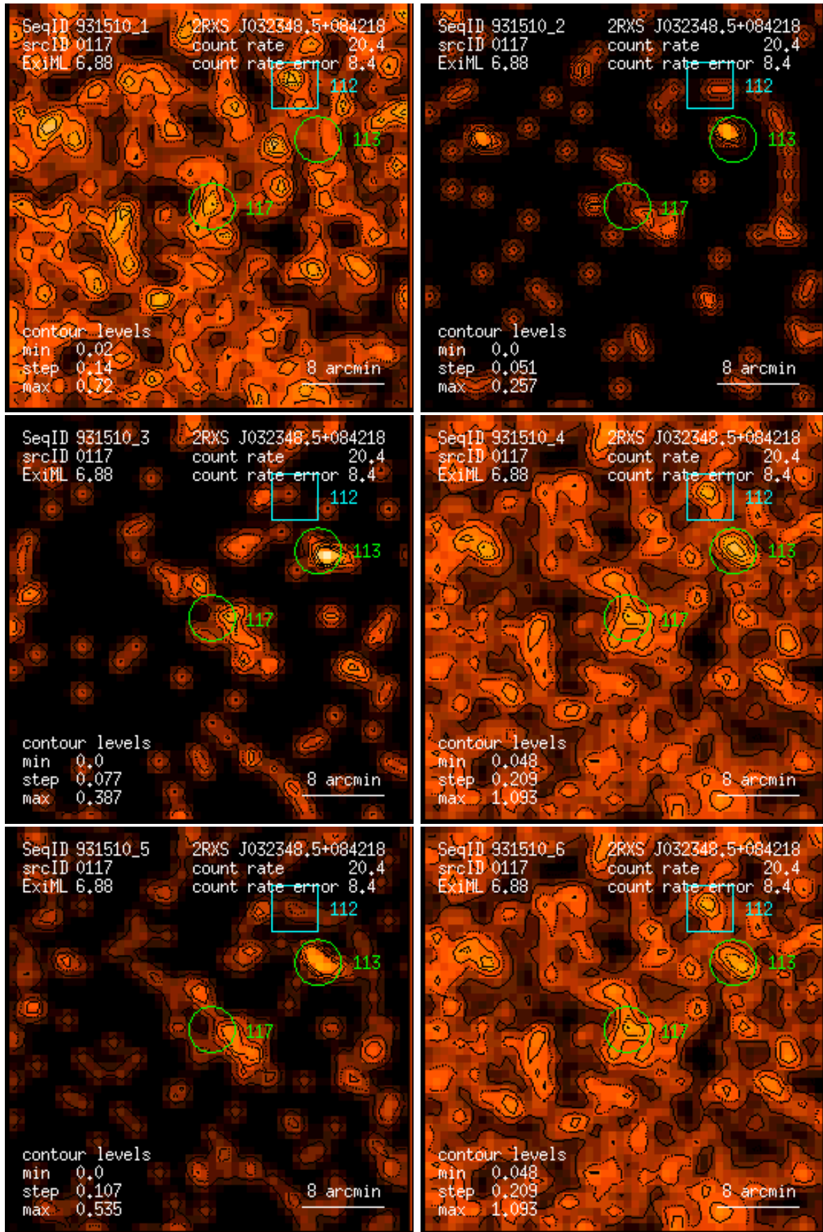
Figure 117: RASS 931510: detection 0117: band rate images, Gaussian filter: (1) PSPC channels 11 – 41, (2) 52 – 90, (3) 91 – 201, (4) 11 – 235, (5) 52 – 201, (6) 11 – 201. Broad band rates in counts/ks. Band rate contour levels in counts/ks/arcmin 2 .
