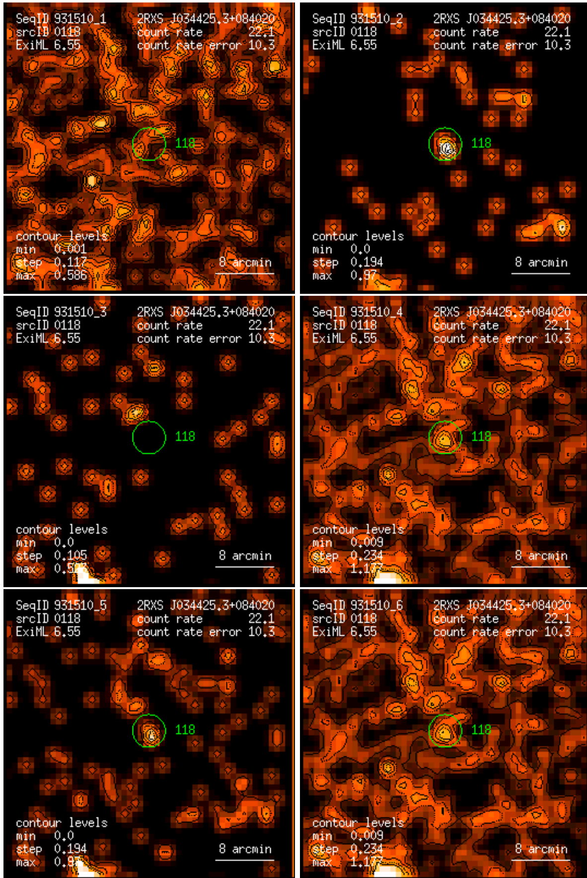
Figure 118: RASS 931510: detection 0118: band rate images, Gaussian filter: (1) PSPC channels 11 – 41, (2) 52 – 90, (3) 91 – 201, (4) 11 – 235, (5) 52 – 201, (6) 11 – 201. Broad band rates in counts/ks. Band rate contour levels in counts/ks/arcmin 2 .
