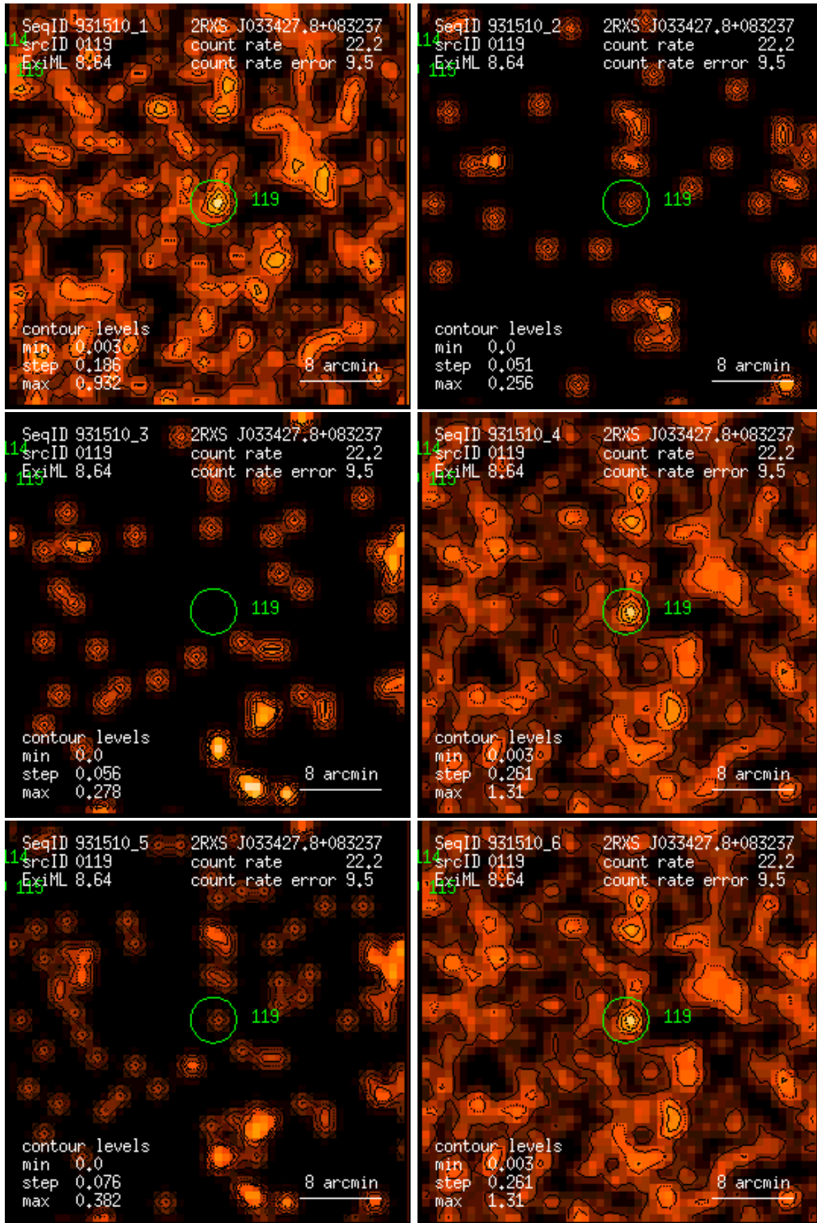
Figure 119: RASS 931510: detection 0119: band rate images, Gaussian filter: (1) PSPC channels 11 – 41, (2) 52 – 90, (3) 91 – 201, (4) 11 – 235, (5) 52 – 201, (6) 11 – 201. Broad band rates in counts/ks. Band rate contour levels in counts/ks/arcmin 2 .
