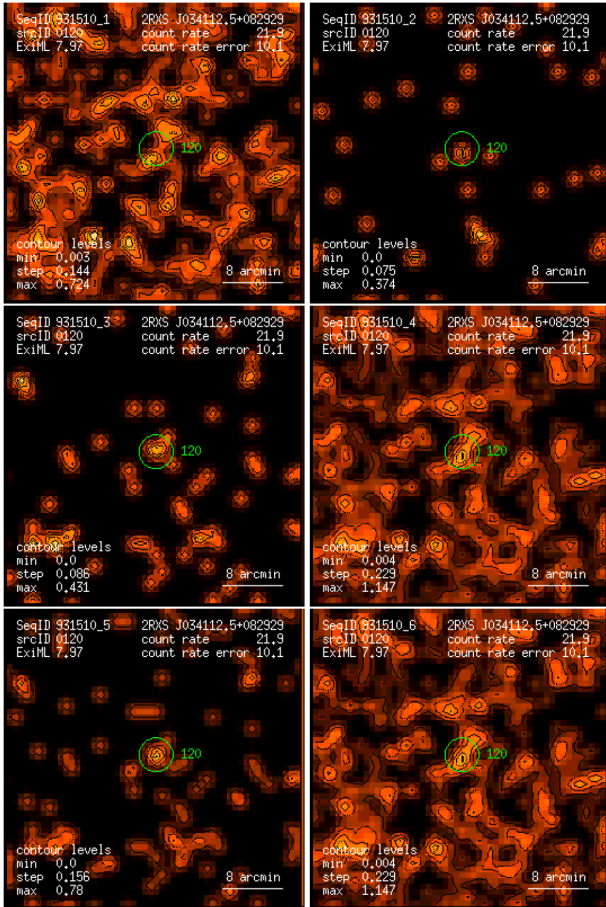
Figure 120: RASS 931510: detection 0120: band rate images, Gaussian filter: (1) PSPC channels 11 – 41, (2) 52 – 90, (3) 91 – 201, (4) 11 – 235, (5) 52 – 201, (6) 11 – 201. Broad band rates in counts/ks. Band rate contour levels in counts/ks/arcmin 2 .
