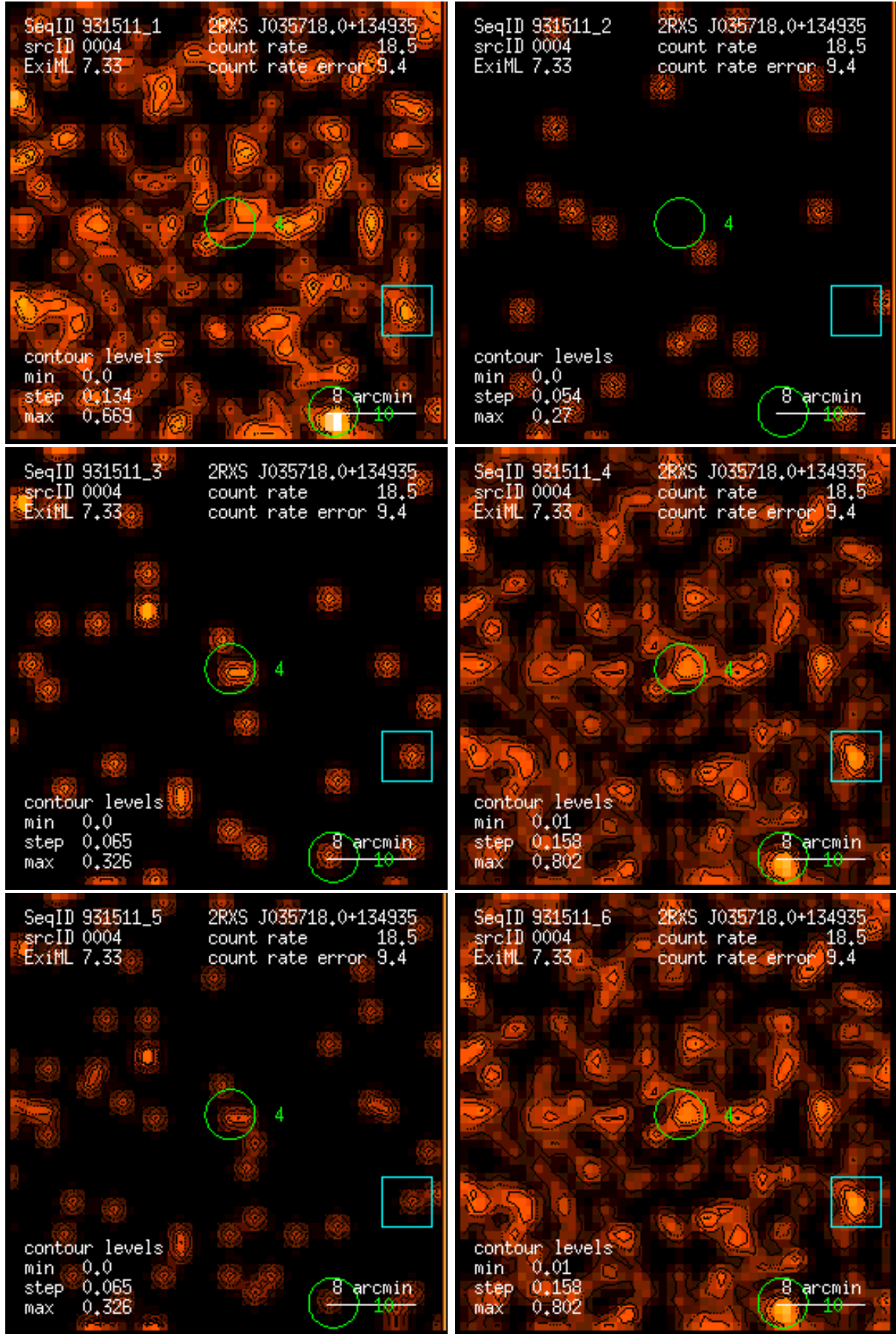
Figure 4: RASS 931511: detection 0004: band rate images, Gaussian filter: (1) PSPC channels 11 – 41, (2) 52 – 90, (3) 91 – 201, (4) 11 – 235, (5) 52 – 201, (6) 11 – 201. Broad band rates in counts/ks. Band rate contour levels in counts/ks/arcmin 2 .
