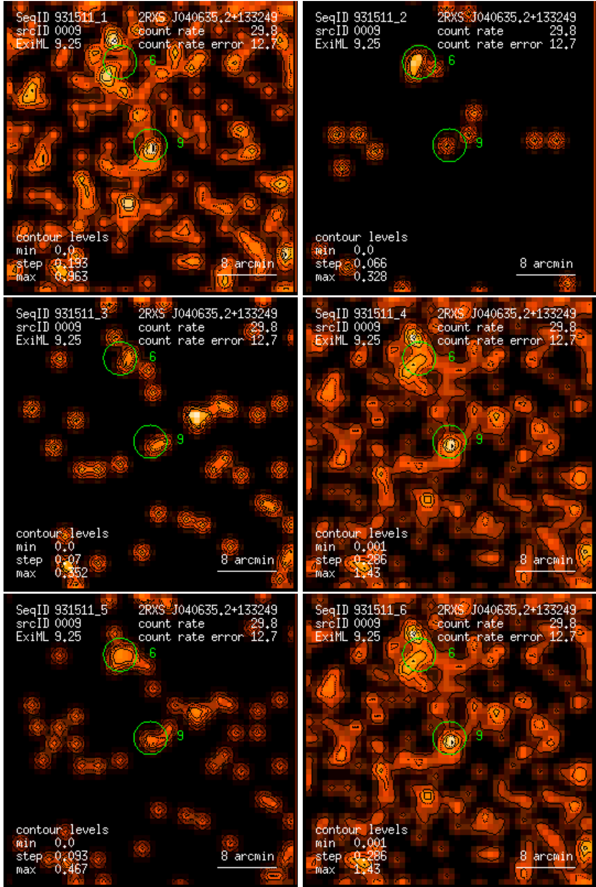
Figure 9: RASS 931511: detection 0009: band rate images, Gaussian filter: (1) PSPC channels 11 – 41, (2) 52 – 90, (3) 91 – 201, (4) 11 – 235, (5) 52 – 201, (6) 11 – 201. Broad band rates in counts/ks. Band rate contour levels in counts/ks/arcmin 2 .
