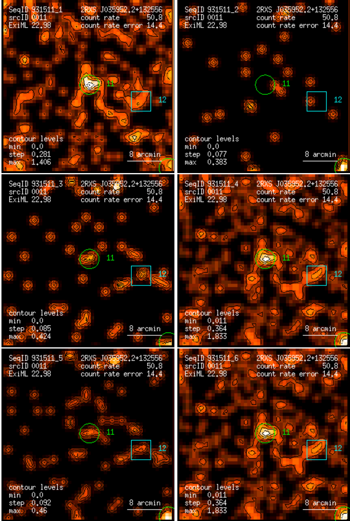
Figure 11: RASS 931511: detection 0011: band rate images, Gaussian filter: (1) PSPC channels 11 – 41, (2) 52 – 90, (3) 91 – 201, (4) 11 – 235, (5) 52 – 201, (6) 11 – 201. Broad band rates in counts/ks. Band rate contour levels in counts/ks/arcmin 2 .
