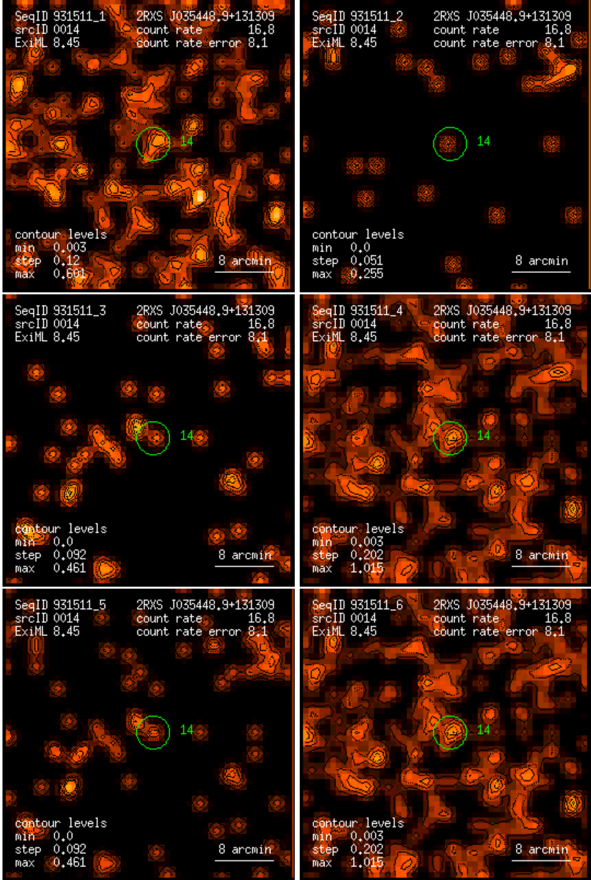
Figure 14: RASS 931511: detection 0014: band rate images, Gaussian filter: (1) PSPC channels 11 – 41, (2) 52 – 90, (3) 91 – 201, (4) 11 – 235, (5) 52 – 201, (6) 11 – 201. Broad band rates in counts/ks. Band rate contour levels in counts/ks/arcmin 2 .
