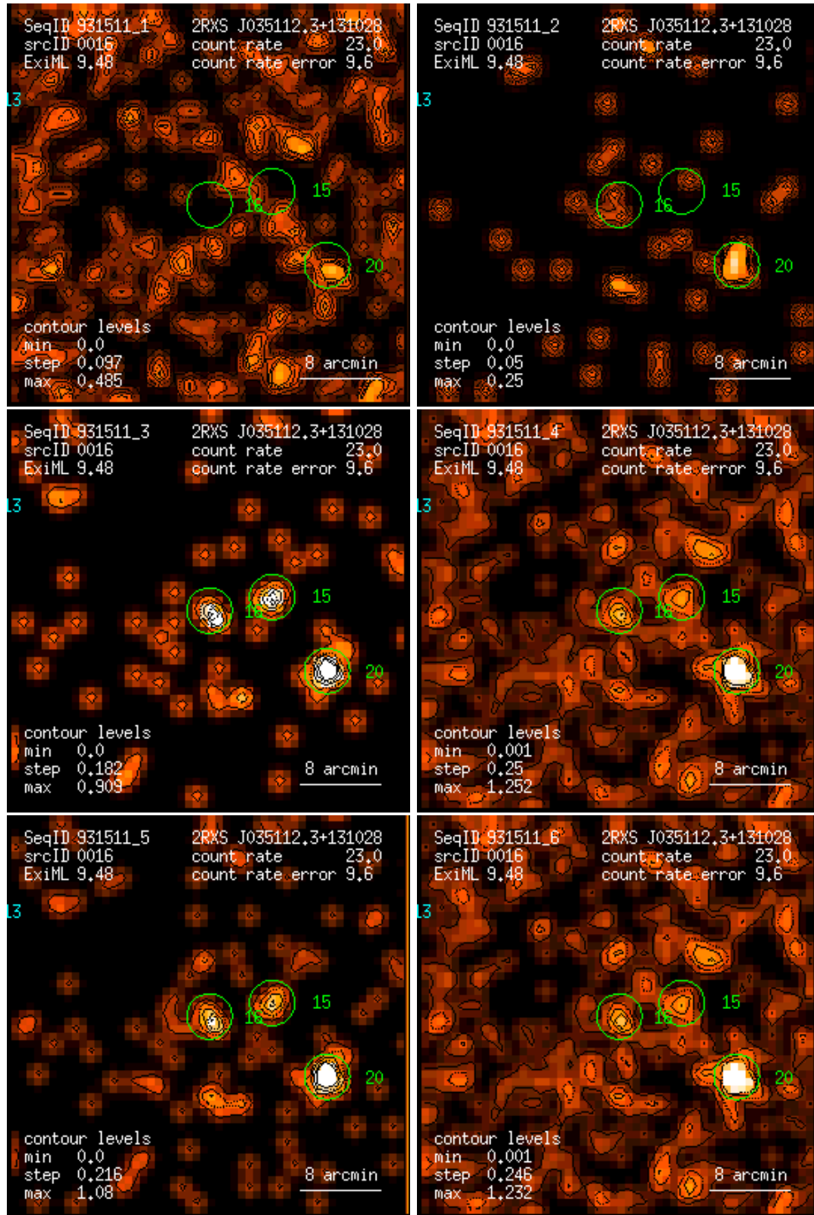
Figure 16: RASS 931511: detection 0016: band rate images, Gaussian filter: (1) PSPC channels 11 – 41, (2) 52 – 90, (3) 91 – 201, (4) 11 – 235, (5) 52 – 201, (6) 11 – 201. Broad band rates in counts/ks. Band rate contour levels in counts/ks/arcmin 2 .
