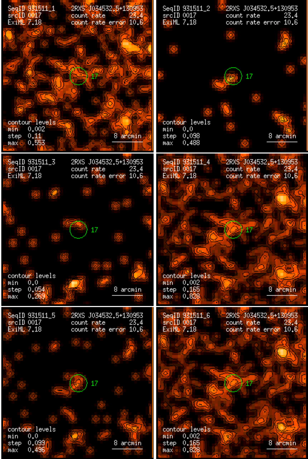
Figure 17: RASS 931511: detection 0017: band rate images, Gaussian filter: (1) PSPC channels 11 – 41, (2) 52 – 90, (3) 91 – 201, (4) 11 – 235, (5) 52 – 201, (6) 11 – 201. Broad band rates in counts/ks. Band rate contour levels in counts/ks/arcmin 2 .
