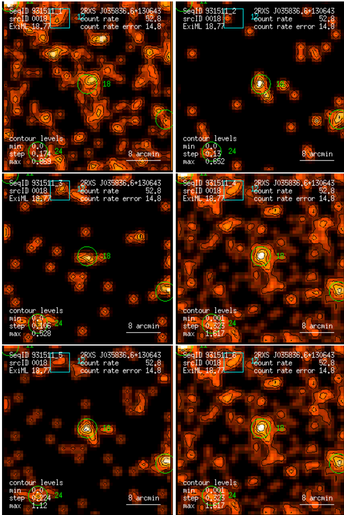
Figure 18: RASS 931511: detection 0018: band rate images, Gaussian filter: (1) PSPC channels 11 – 41, (2) 52 – 90, (3) 91 – 201, (4) 11 – 235, (5) 52 – 201, (6) 11 – 201. Broad band rates in counts/ks. Band rate contour levels in counts/ks/arcmin 2 .
