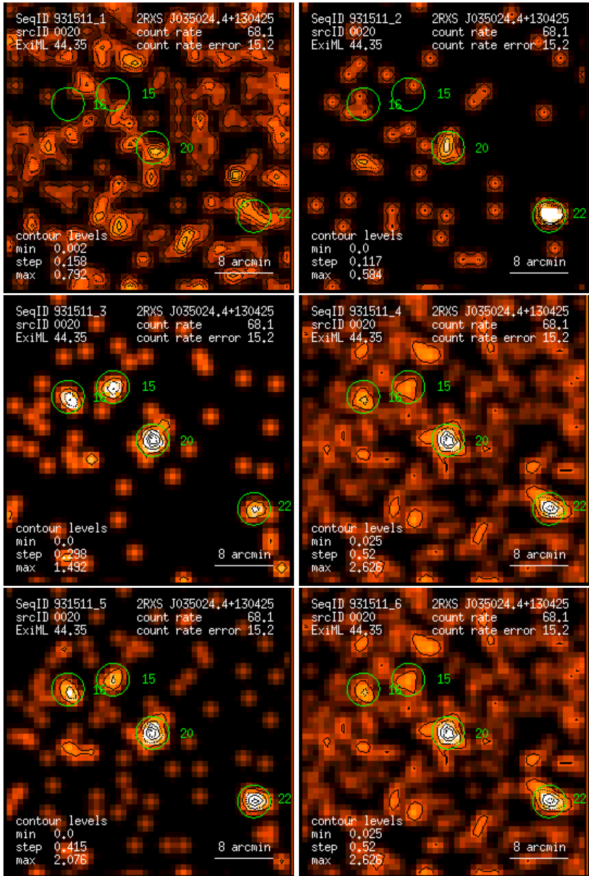
Figure 20: RASS 931511: detection 0020: band rate images, Gaussian filter: (1) PSPC channels 11 – 41, (2) 52 – 90, (3) 91 – 201, (4) 11 – 235, (5) 52 – 201, (6) 11 – 201. Broad band rates in counts/ks. Band rate contour levels in counts/ks/arcmin 2 .
