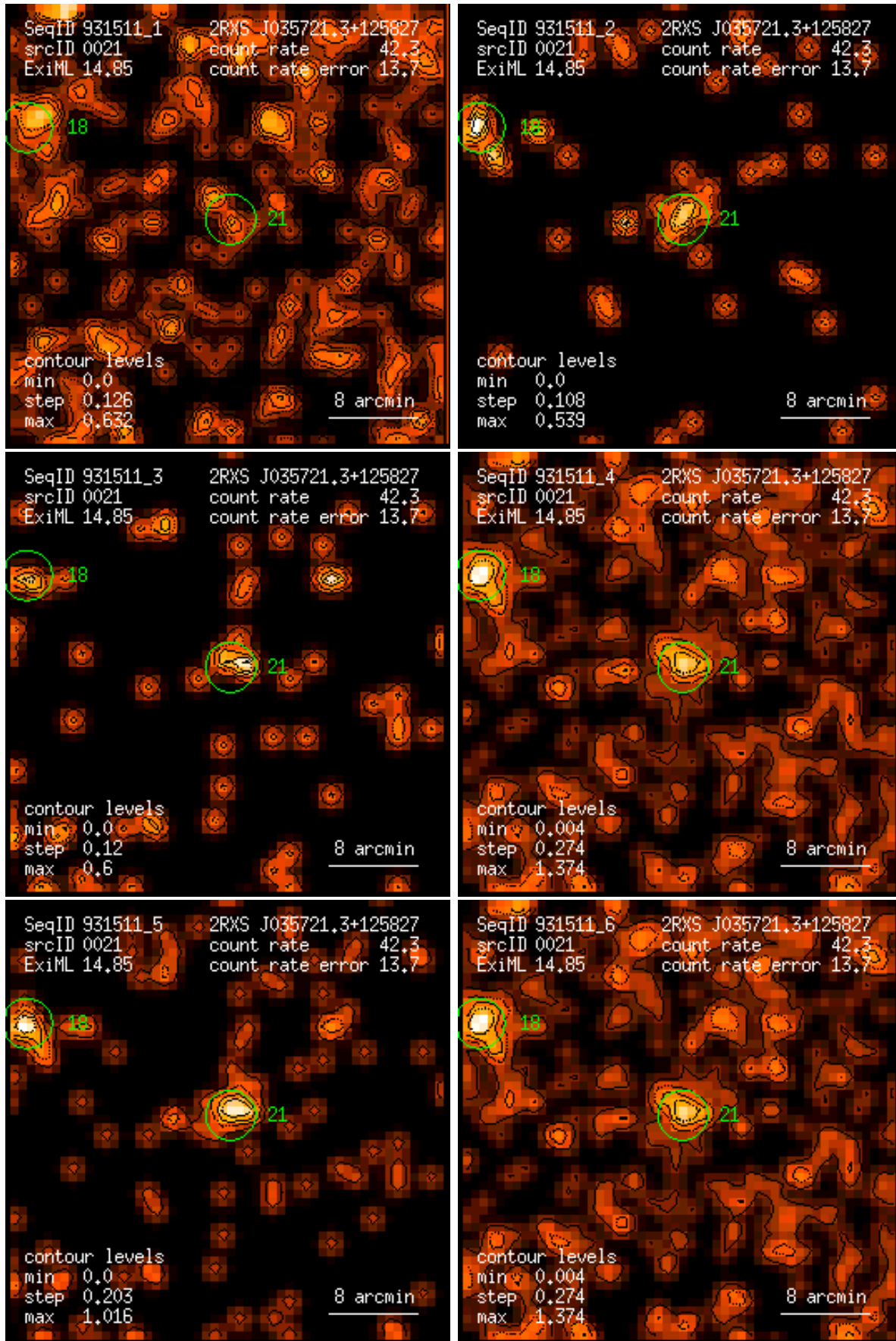
Figure 21: RASS 931511: detection 0021: band rate images, Gaussian filter: (1) PSPC channels 11 – 41, (2) 52 – 90, (3) 91 – 201, (4) 11 – 235, (5) 52 – 201, (6) 11 – 201. Broad band rates in counts/ks. Band rate contour levels in counts/ks/arcmin 2 .
