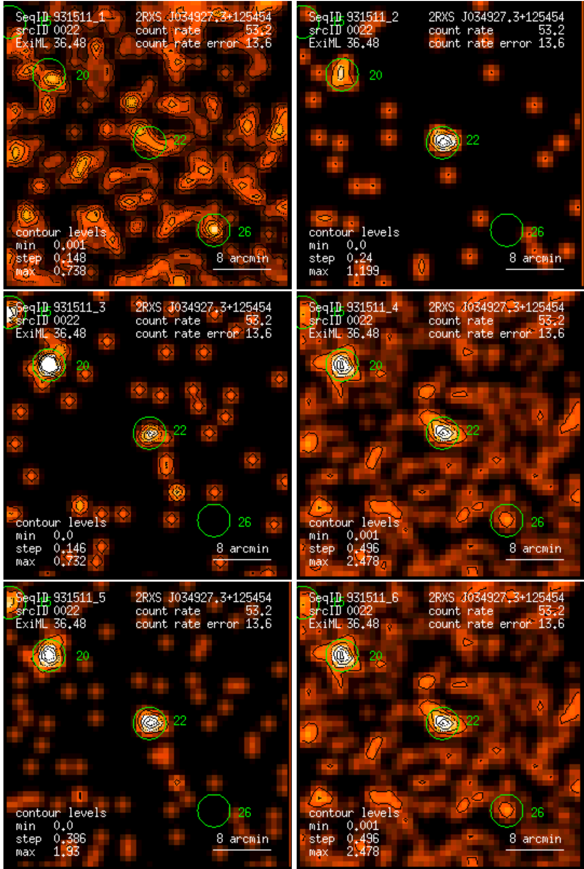
Figure 22: RASS 931511: detection 0022: band rate images, Gaussian filter: (1) PSPC channels 11 – 41, (2) 52 – 90, (3) 91 – 201, (4) 11 – 235, (5) 52 – 201, (6) 11 – 201. Broad band rates in counts/ks. Band rate contour levels in counts/ks/arcmin 2 .
