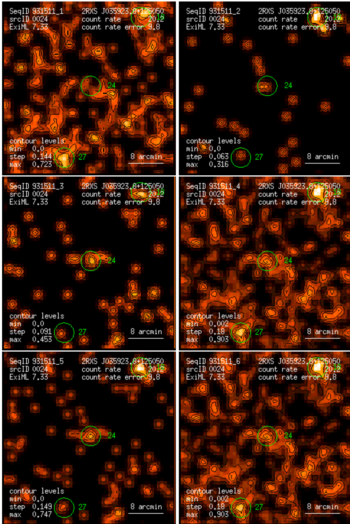
Figure 24: RASS 931511: detection 0024: band rate images, Gaussian filter: (1) PSPC channels 11 – 41, (2) 52 – 90, (3) 91 – 201, (4) 11 – 235, (5) 52 – 201, (6) 11 – 201. Broad band rates in counts/ks. Band rate contour levels in counts/ks/arcmin 2 .
