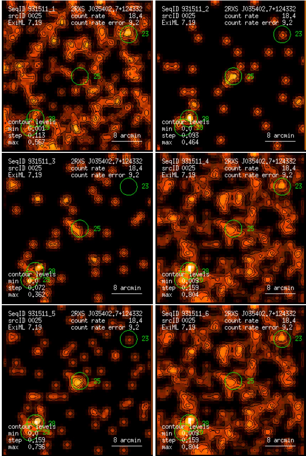
Figure 25: RASS 931511: detection 0025: band rate images, Gaussian filter: (1) PSPC channels 11 – 41, (2) 52 – 90, (3) 91 – 201, (4) 11 – 235, (5) 52 – 201, (6) 11 – 201. Broad band rates in counts/ks. Band rate contour levels in counts/ks/arcmin 2 .
