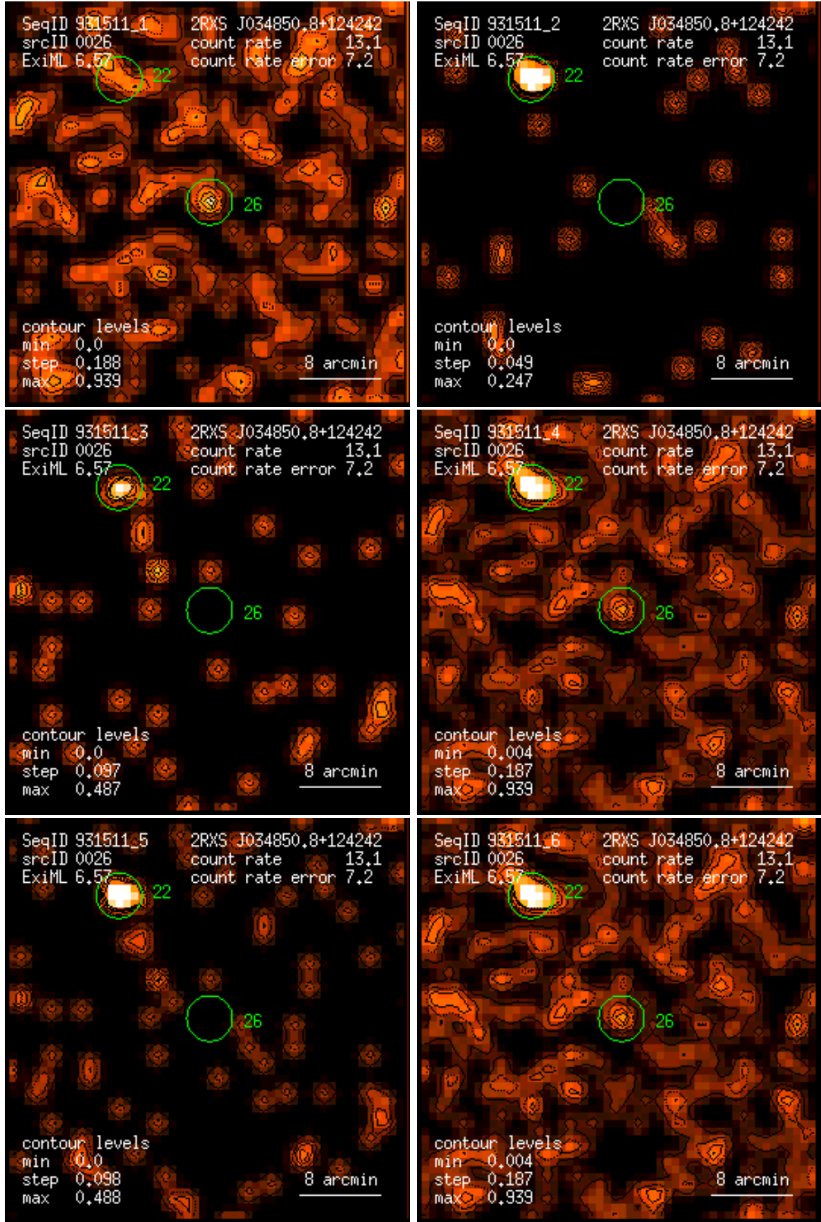
Figure 26: RASS 931511: detection 0026: band rate images, Gaussian filter: (1) PSPC channels 11 – 41, (2) 52 – 90, (3) 91 – 201, (4) 11 – 235, (5) 52 – 201, (6) 11 – 201. Broad band rates in counts/ks. Band rate contour levels in counts/ks/arcmin 2 .
