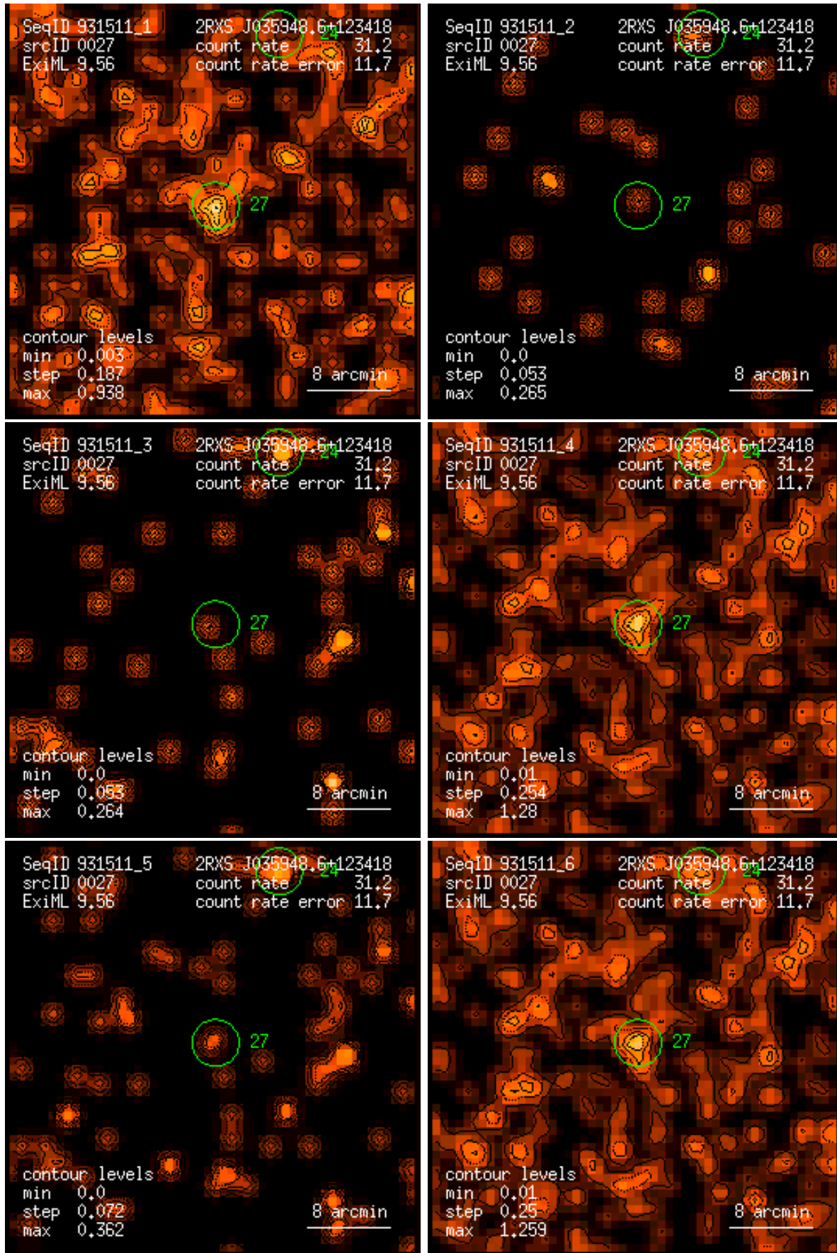
Figure 27: RASS 931511: detection 0027: band rate images, Gaussian filter: (1) PSPC channels 11 – 41, (2) 52 – 90, (3) 91 – 201, (4) 11 – 235, (5) 52 – 201, (6) 11 – 201. Broad band rates in counts/ks. Band rate contour levels in counts/ks/arcmin 2 .
