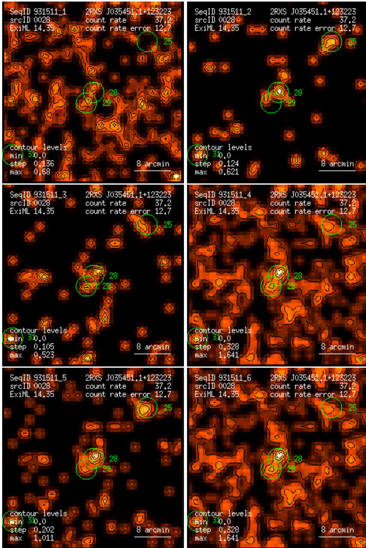
Figure 28: RASS 931511: detection 0028: band rate images, Gaussian filter: (1) PSPC channels 11 – 41, (2) 52 – 90, (3) 91 – 201, (4) 11 – 235, (5) 52 – 201, (6) 11 – 201. Broad band rates in counts/ks. Band rate contour levels in counts/ks/arcmin 2 .
