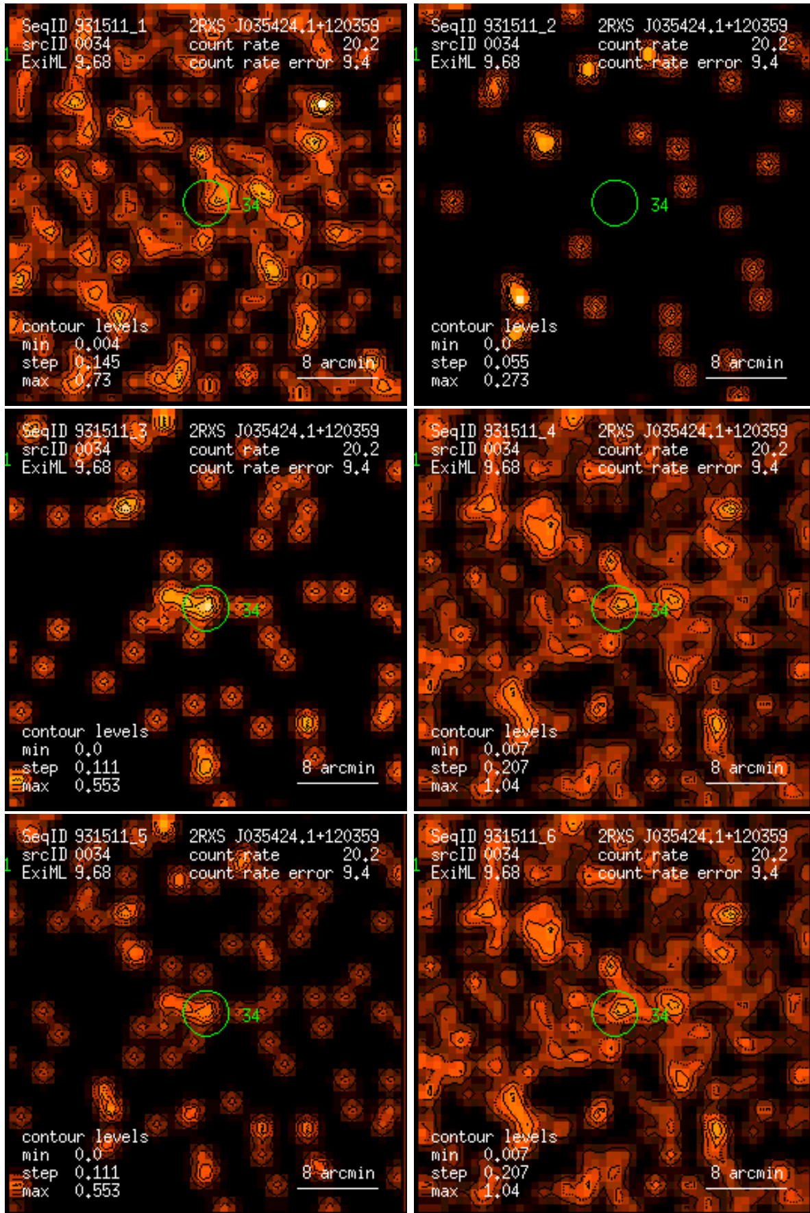
Figure 34: RASS 931511: detection 0034: band rate images, Gaussian filter: (1) PSPC channels 11 – 41, (2) 52 – 90, (3) 91 – 201, (4) 11 – 235, (5) 52 – 201, (6) 11 – 201. Broad band rates in counts/ks. Band rate contour levels in counts/ks/arcmin 2 .
