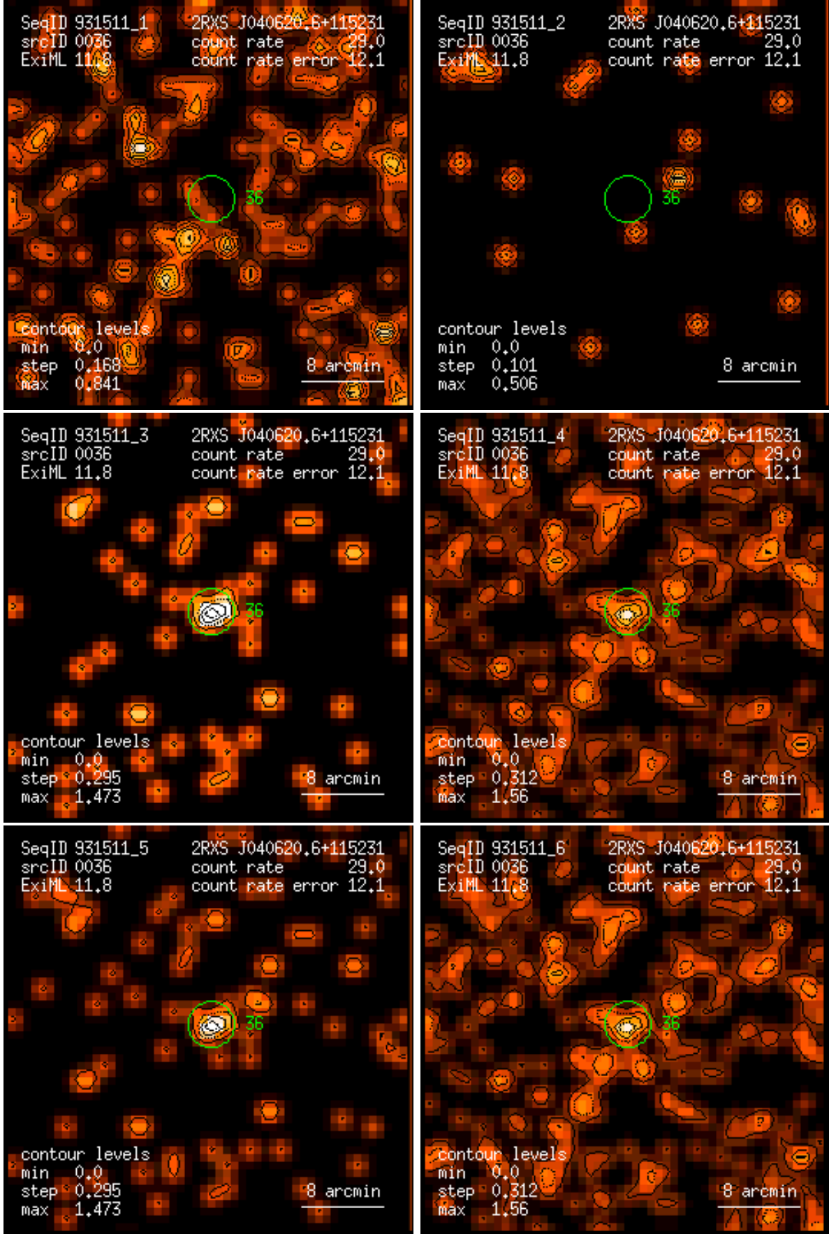
Figure 36: RASS 931511: detection 0036: band rate images, Gaussian filter: (1) PSPC channels 11 – 41, (2) 52 – 90, (3) 91 – 201, (4) 11 – 235, (5) 52 – 201, (6) 11 – 201. Broad band rates in counts/ks. Band rate contour levels in counts/ks/arcmin 2 .
