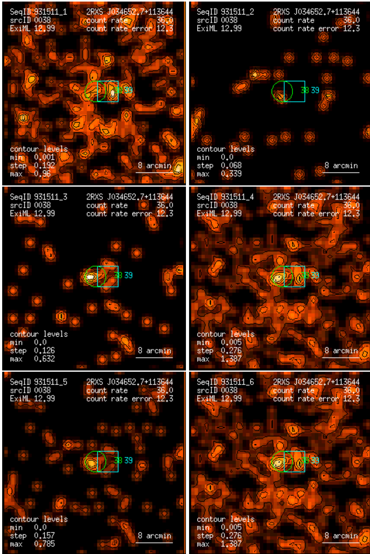
Figure 38: RASS 931511: detection 0038: band rate images, Gaussian filter: (1) PSPC channels 11 – 41, (2) 52 – 90, (3) 91 – 201, (4) 11 – 235, (5) 52 – 201, (6) 11 – 201. Broad band rates in counts/ks. Band rate contour levels in counts/ks/arcmin 2 .
