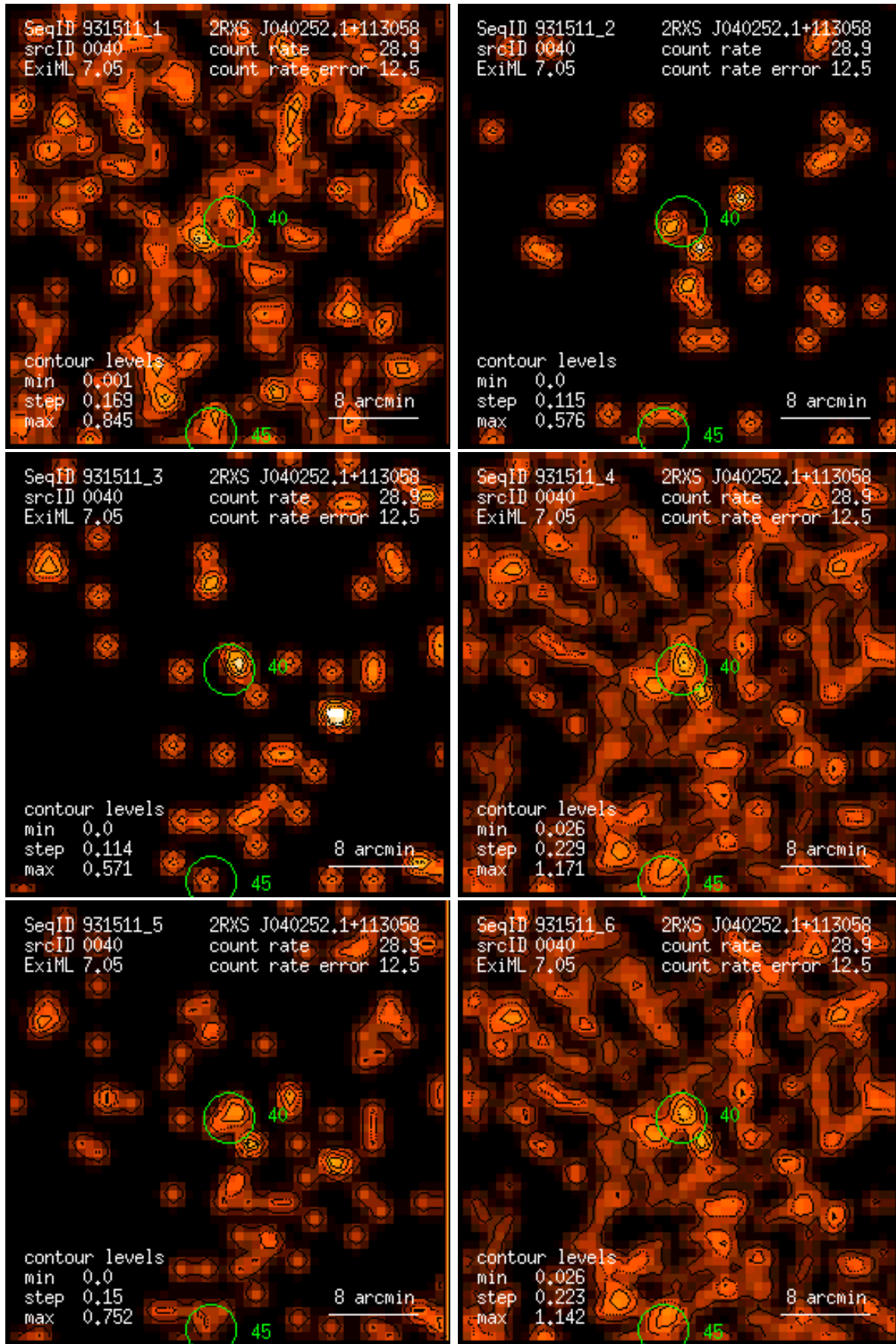
Figure 40: RASS 931511: detection 0040: band rate images, Gaussian filter: (1) PSPC channels 11 – 41, (2) 52 – 90, (3) 91 – 201, (4) 11 – 235, (5) 52 – 201, (6) 11 – 201. Broad band rates in counts/ks. Band rate contour levels in counts/ks/arcmin 2 .
