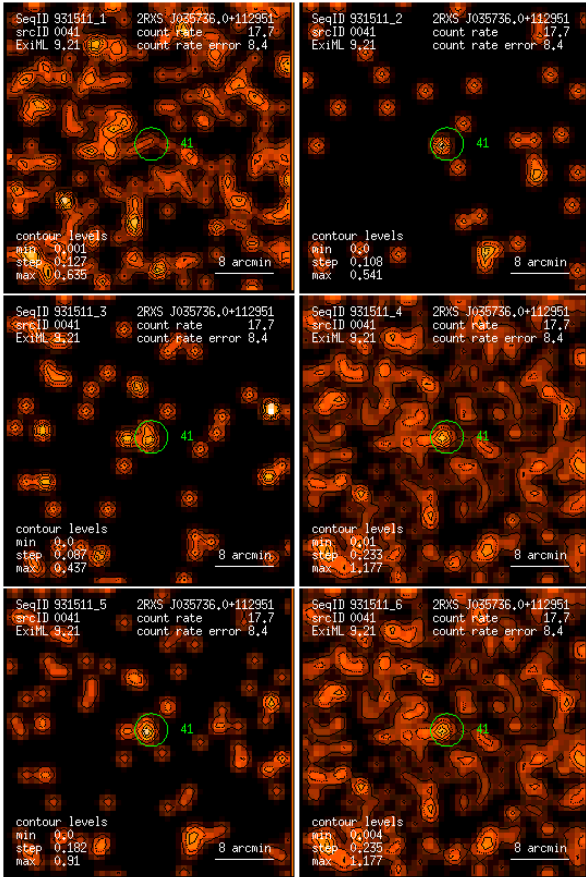
Figure 41: RASS 931511: detection 0041: band rate images, Gaussian filter: (1) PSPC channels 11 – 41, (2) 52 – 90, (3) 91 – 201, (4) 11 – 235, (5) 52 – 201, (6) 11 – 201. Broad band rates in counts/ks. Band rate contour levels in counts/ks/arcmin 2 .
