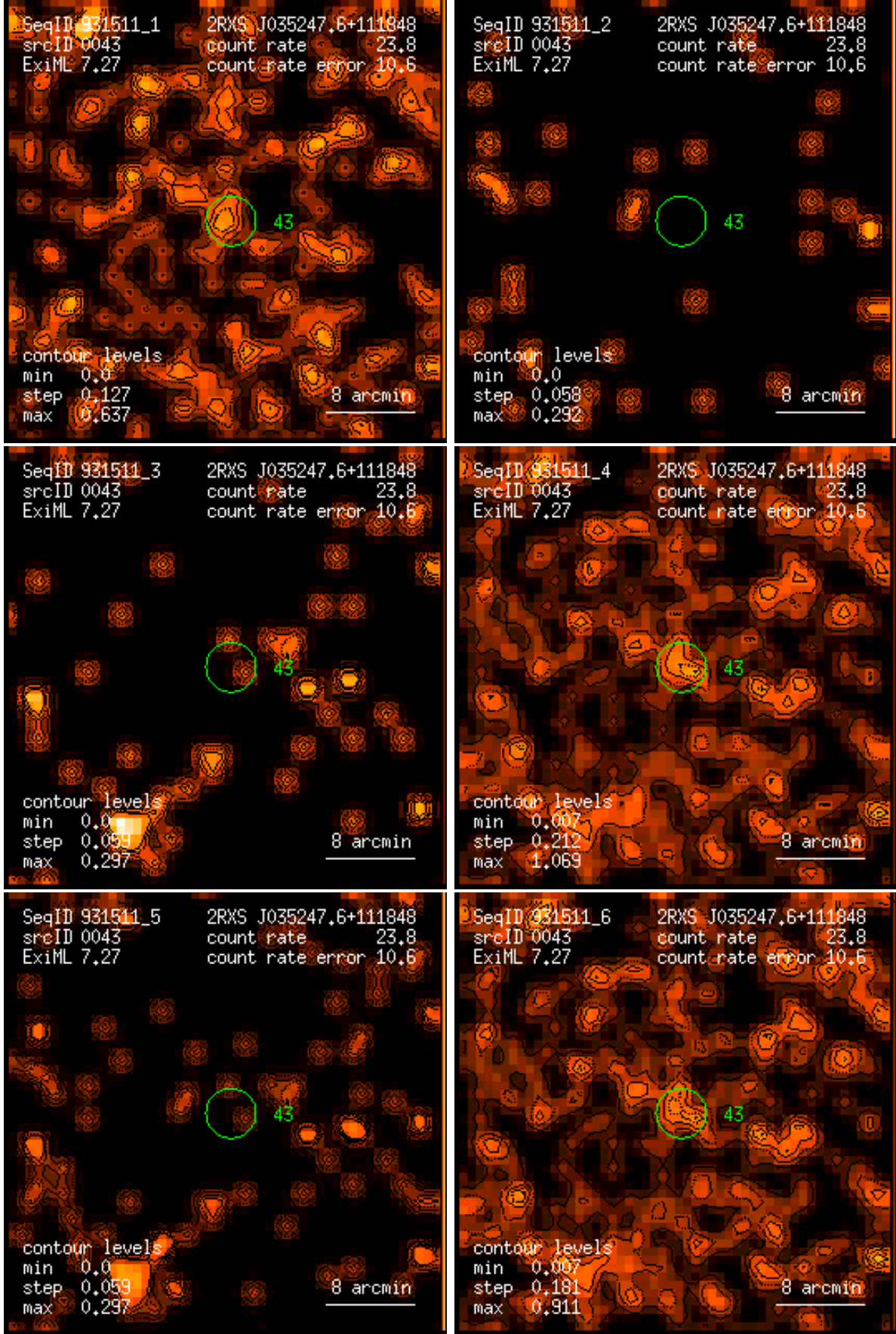
Figure 43: RASS 931511: detection 0043: band rate images, Gaussian filter: (1) PSPC channels 11 – 41, (2) 52 – 90, (3) 91 – 201, (4) 11 – 235, (5) 52 – 201, (6) 11 – 201. Broad band rates in counts/ks. Band rate contour levels in counts/ks/arcmin 2 .
