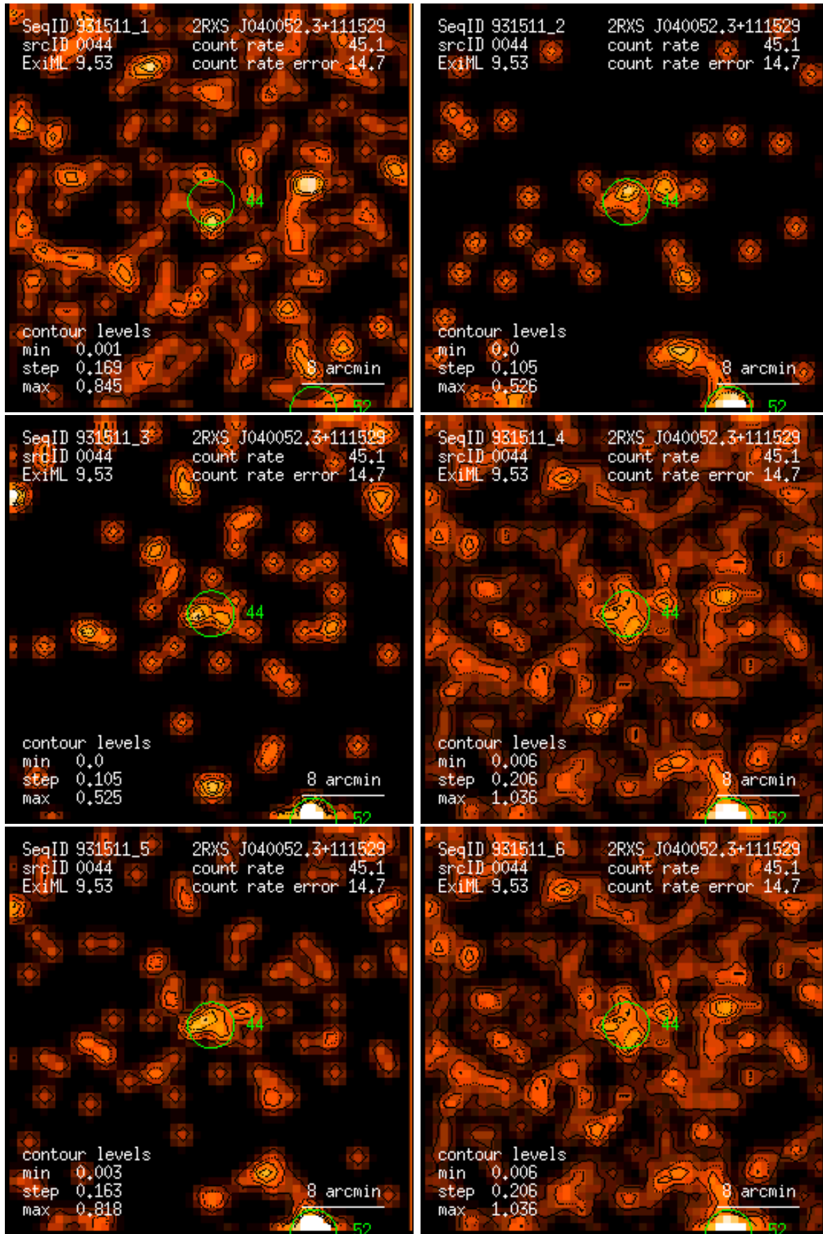
Figure 44: RASS 931511: detection 0044: band rate images, Gaussian filter: (1) PSPC channels 11 – 41, (2) 52 – 90, (3) 91 – 201, (4) 11 – 235, (5) 52 – 201, (6) 11 – 201. Broad band rates in counts/ks. Band rate contour levels in counts/ks/arcmin 2 .
