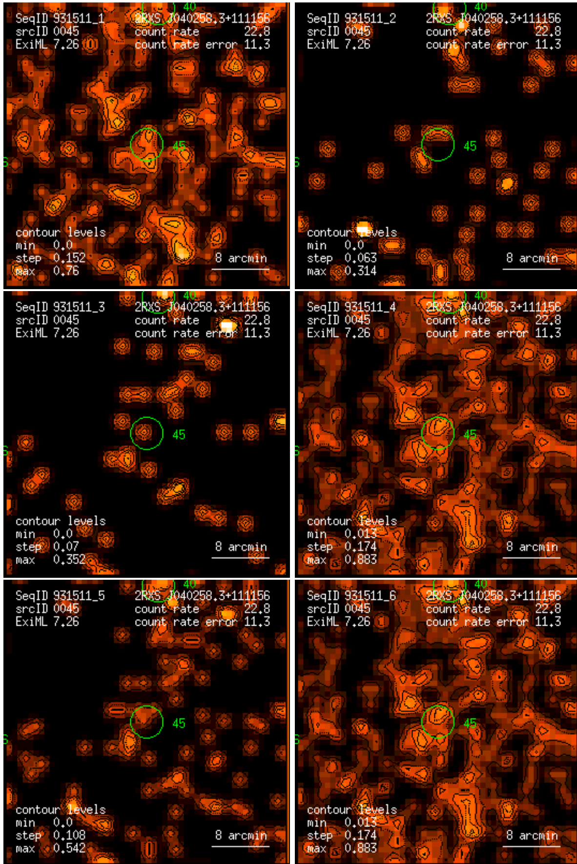
Figure 45: RASS 931511: detection 0045: band rate images, Gaussian filter: (1) PSPC channels 11 – 41, (2) 52 – 90, (3) 91 – 201, (4) 11 – 235, (5) 52 – 201, (6) 11 – 201. Broad band rates in counts/ks. Band rate contour levels in counts/ks/arcmin 2 .
