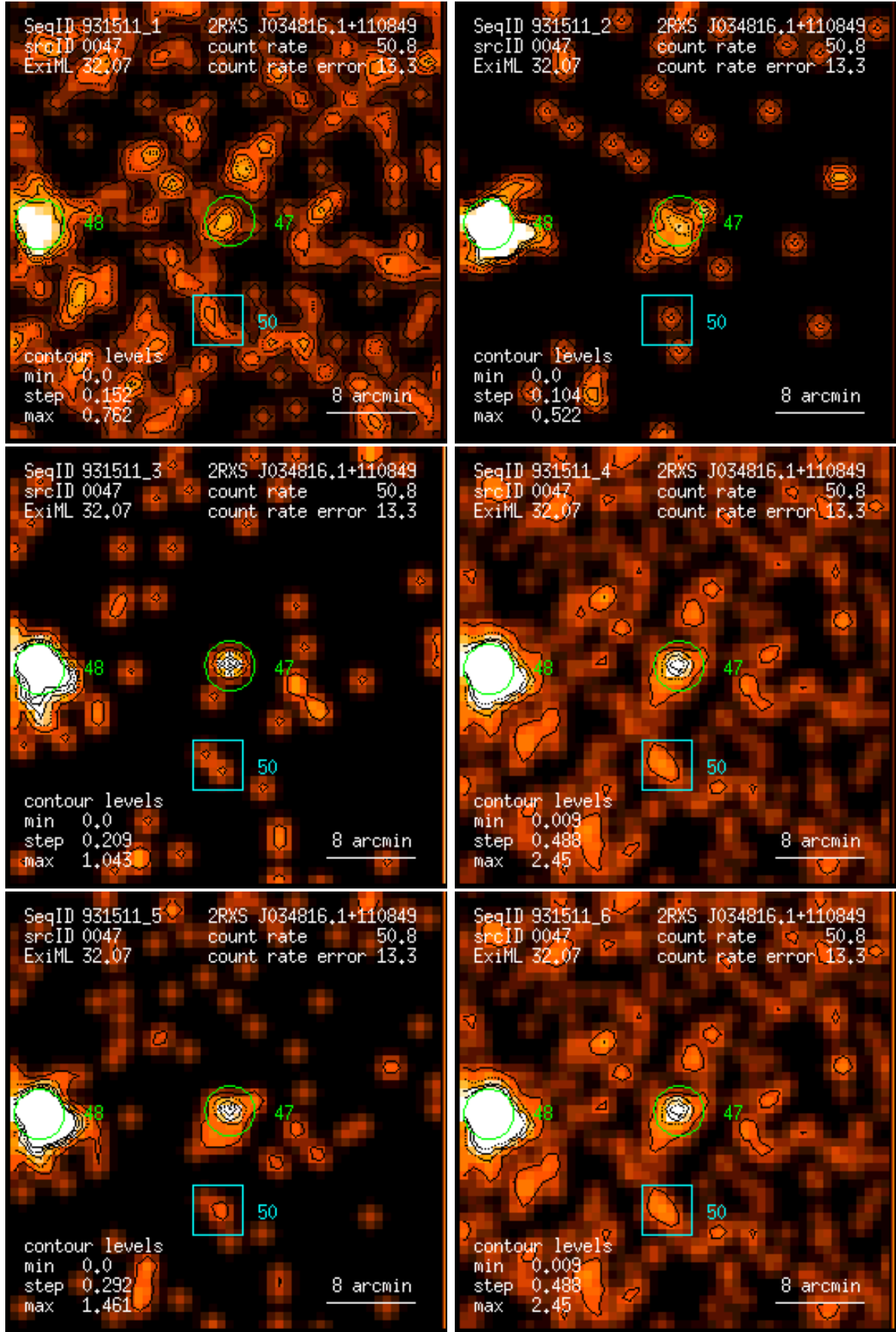
Figure 47: RASS 931511: detection 0047: band rate images, Gaussian filter: (1) PSPC channels 11 – 41, (2) 52 – 90, (3) 91 – 201, (4) 11 – 235, (5) 52 – 201, (6) 11 – 201. Broad band rates in counts/ks. Band rate contour levels in counts/ks/arcmin 2 .
