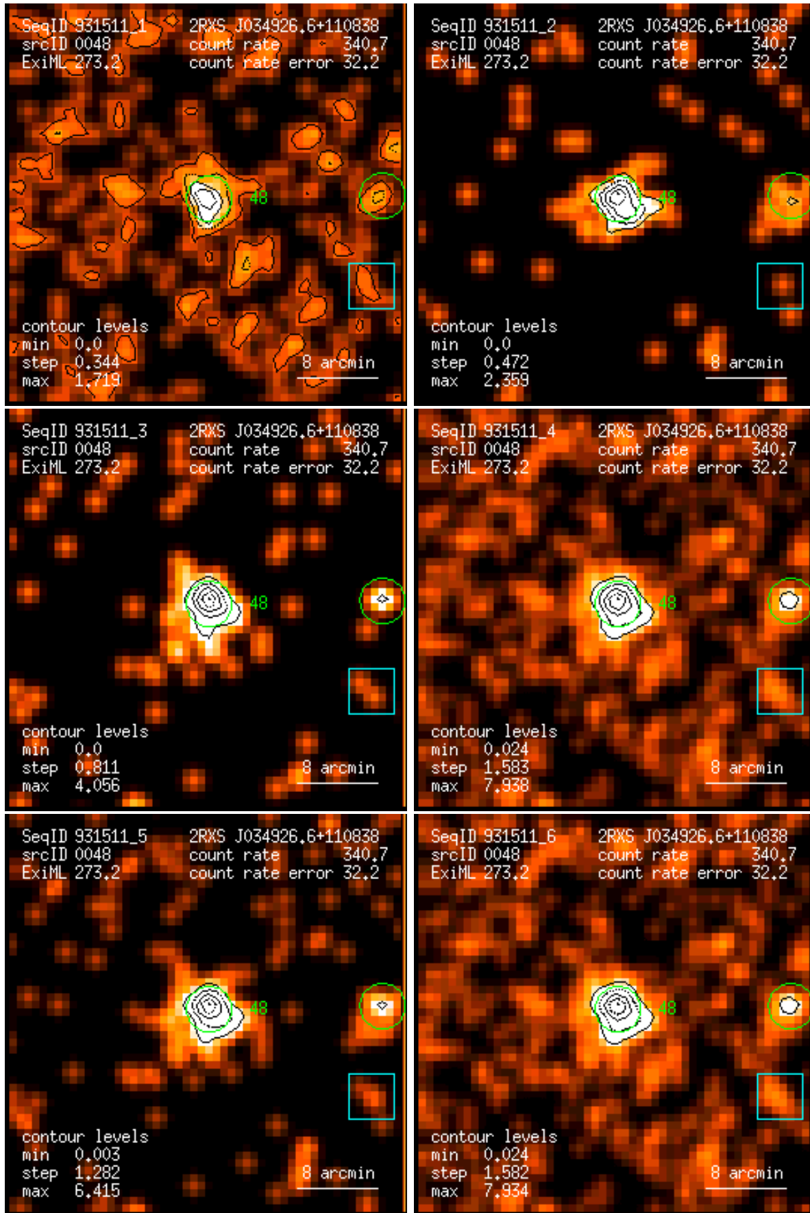
Figure 48: RASS 931511: detection 0048: band rate images, Gaussian filter: (1) PSPC channels 11 – 41, (2) 52 – 90, (3) 91 – 201, (4) 11 – 235, (5) 52 – 201, (6) 11 – 201. Broad band rates in counts/ks. Band rate contour levels in counts/ks/arcmin 2 .
