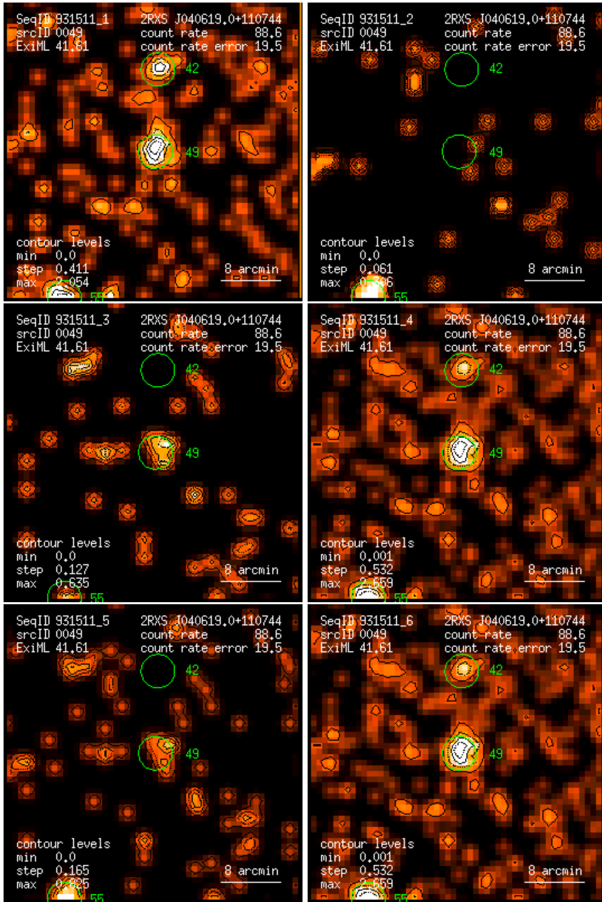
Figure 49: RASS 931511: detection 0049: band rate images, Gaussian filter: (1) PSPC channels 11 – 41, (2) 52 – 90, (3) 91 – 201, (4) 11 – 235, (5) 52 – 201, (6) 11 – 201. Broad band rates in counts/ks. Band rate contour levels in counts/ks/arcmin 2 .
