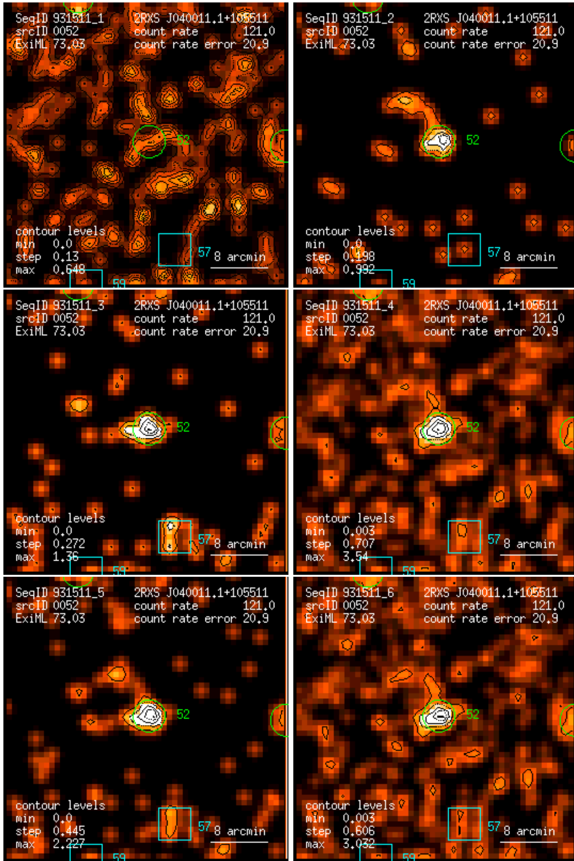
Figure 52: RASS 931511: detection 0052: band rate images, Gaussian filter: (1) PSPC channels 11 – 41, (2) 52 – 90, (3) 91 – 201, (4) 11 – 235, (5) 52 – 201, (6) 11 – 201. Broad band rates in counts/ks. Band rate contour levels in counts/ks/arcmin 2 .
