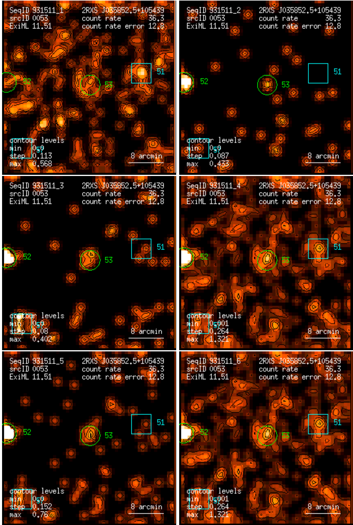
Figure 53: RASS 931511: detection 0053: band rate images, Gaussian filter: (1) PSPC channels 11 – 41, (2) 52 – 90, (3) 91 – 201, (4) 11 – 235, (5) 52 – 201, (6) 11 – 201. Broad band rates in counts/ks. Band rate contour levels in counts/ks/arcmin 2 .
