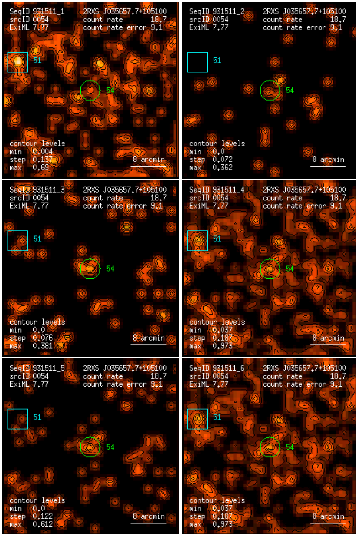
Figure 54: RASS 931511: detection 0054: band rate images, Gaussian filter: (1) PSPC channels 11 – 41, (2) 52 – 90, (3) 91 – 201, (4) 11 – 235, (5) 52 – 201, (6) 11 – 201. Broad band rates in counts/ks. Band rate contour levels in counts/ks/arcmin 2 .
