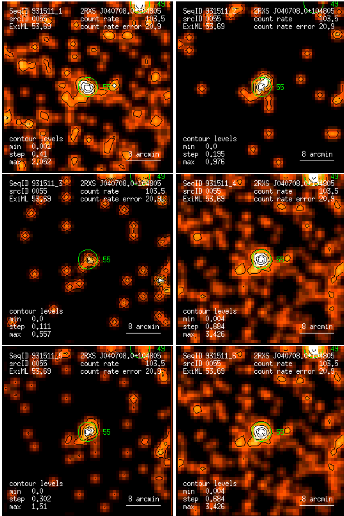
Figure 55: RASS 931511: detection 0055: band rate images, Gaussian filter: (1) PSPC channels 11 – 41, (2) 52 – 90, (3) 91 – 201, (4) 11 – 235, (5) 52 – 201, (6) 11 – 201. Broad band rates in counts/ks. Band rate contour levels in counts/ks/arcmin 2 .
