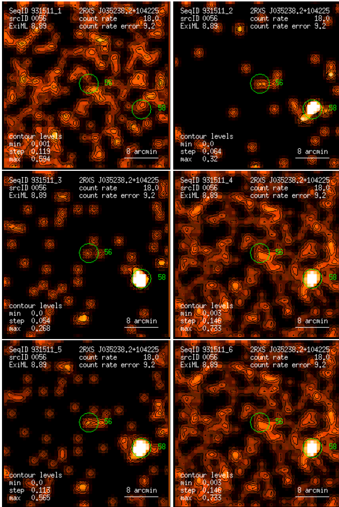
Figure 56: RASS 931511: detection 0056: band rate images, Gaussian filter: (1) PSPC channels 11 – 41, (2) 52 – 90, (3) 91 – 201, (4) 11 – 235, (5) 52 – 201, (6) 11 – 201. Broad band rates in counts/ks. Band rate contour levels in counts/ks/arcmin 2 .
