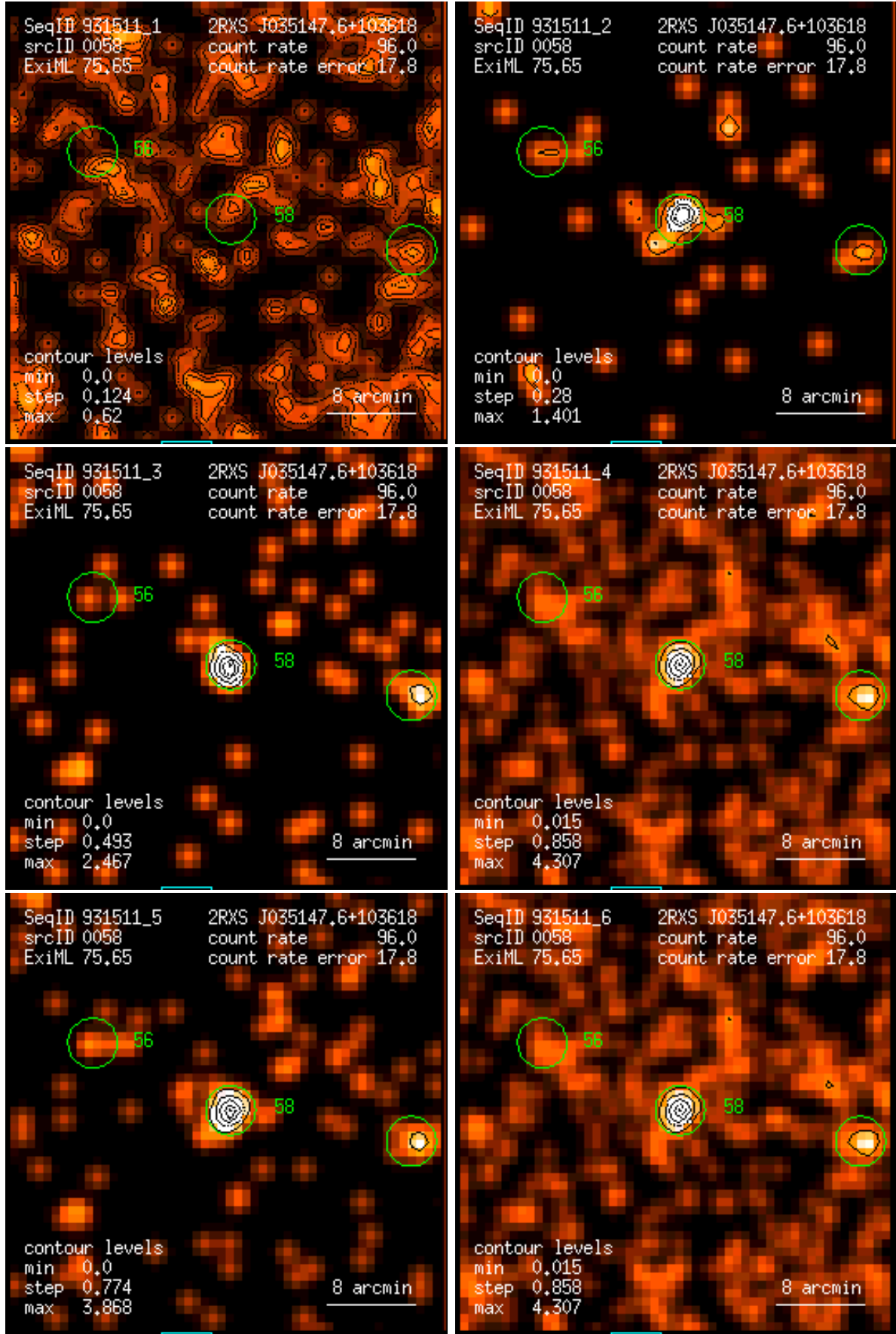
Figure 58: RASS 931511: detection 0058: band rate images, Gaussian filter: (1) PSPC channels 11 – 41, (2) 52 – 90, (3) 91 – 201, (4) 11 – 235, (5) 52 – 201, (6) 11 – 201. Broad band rates in counts/ks. Band rate contour levels in counts/ks/arcmin 2 .
