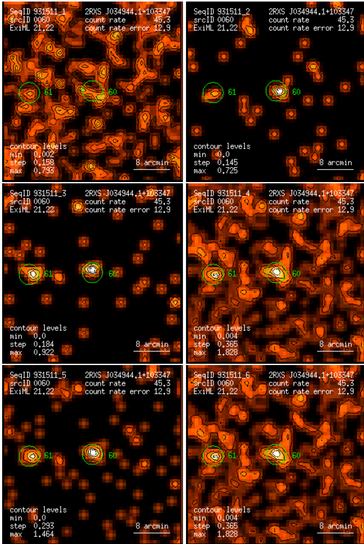
Figure 60: RASS 931511: detection 0060: band rate images, Gaussian filter: (1) PSPC channels 11 – 41, (2) 52 – 90, (3) 91 – 201, (4) 11 – 235, (5) 52 – 201, (6) 11 – 201. Broad band rates in counts/ks. Band rate contour levels in counts/ks/arcmin 2 .
