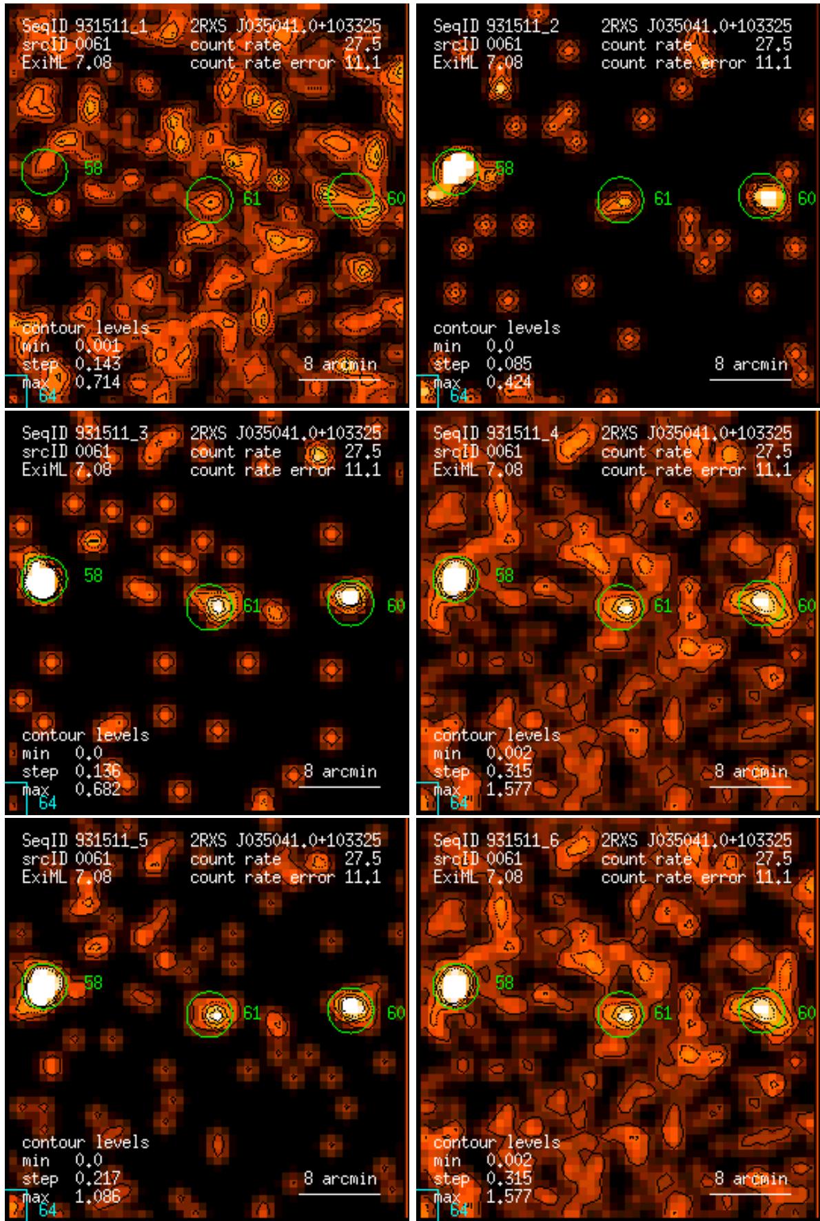
Figure 61: RASS 931511: detection 0061: band rate images, Gaussian filter: (1) PSPC channels 11 – 41, (2) 52 – 90, (3) 91 – 201, (4) 11 – 235, (5) 52 – 201, (6) 11 – 201. Broad band rates in counts/ks. Band rate contour levels in counts/ks/arcmin 2 .
