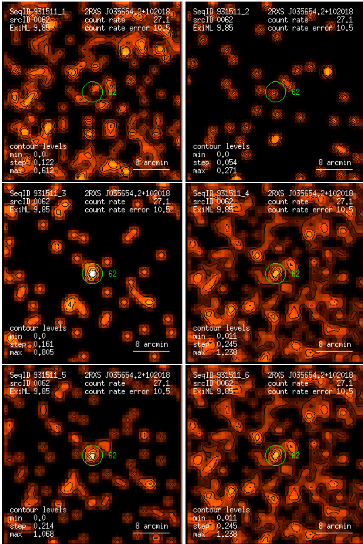
Figure 62: RASS 931511: detection 0062: band rate images, Gaussian filter: (1) PSPC channels 11 – 41, (2) 52 – 90, (3) 91 – 201, (4) 11 – 235, (5) 52 – 201, (6) 11 – 201. Broad band rates in counts/ks. Band rate contour levels in counts/ks/arcmin 2 .
