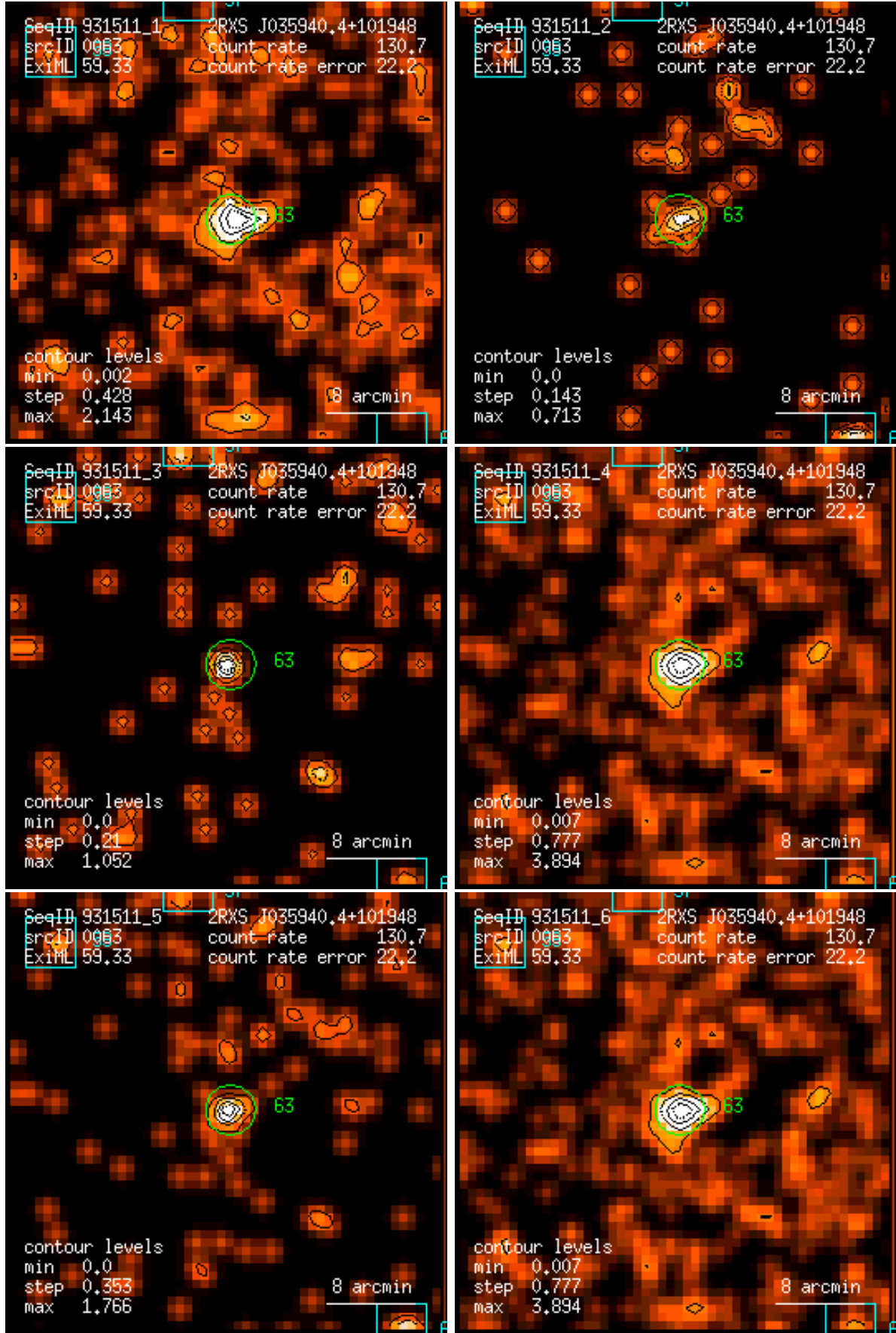
Figure 63: RASS 931511: detection 0063: band rate images, Gaussian filter: (1) PSPC channels 11 – 41, (2) 52 – 90, (3) 91 – 201, (4) 11 – 235, (5) 52 – 201, (6) 11 – 201. Broad band rates in counts/ks. Band rate contour levels in counts/ks/arcmin 2 .
