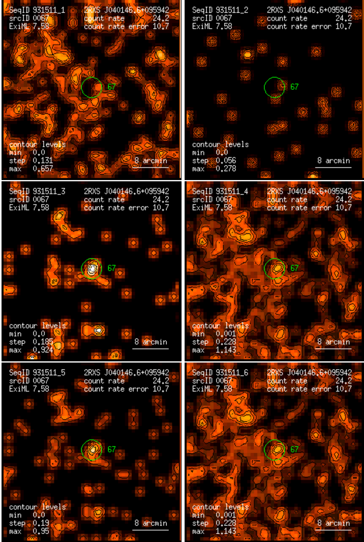
Figure 67: RASS 931511: detection 0067: band rate images, Gaussian filter: (1) PSPC channels 11 – 41, (2) 52 – 90, (3) 91 – 201, (4) 11 – 235, (5) 52 – 201, (6) 11 – 201. Broad band rates in counts/ks. Band rate contour levels in counts/ks/arcmin 2 .
