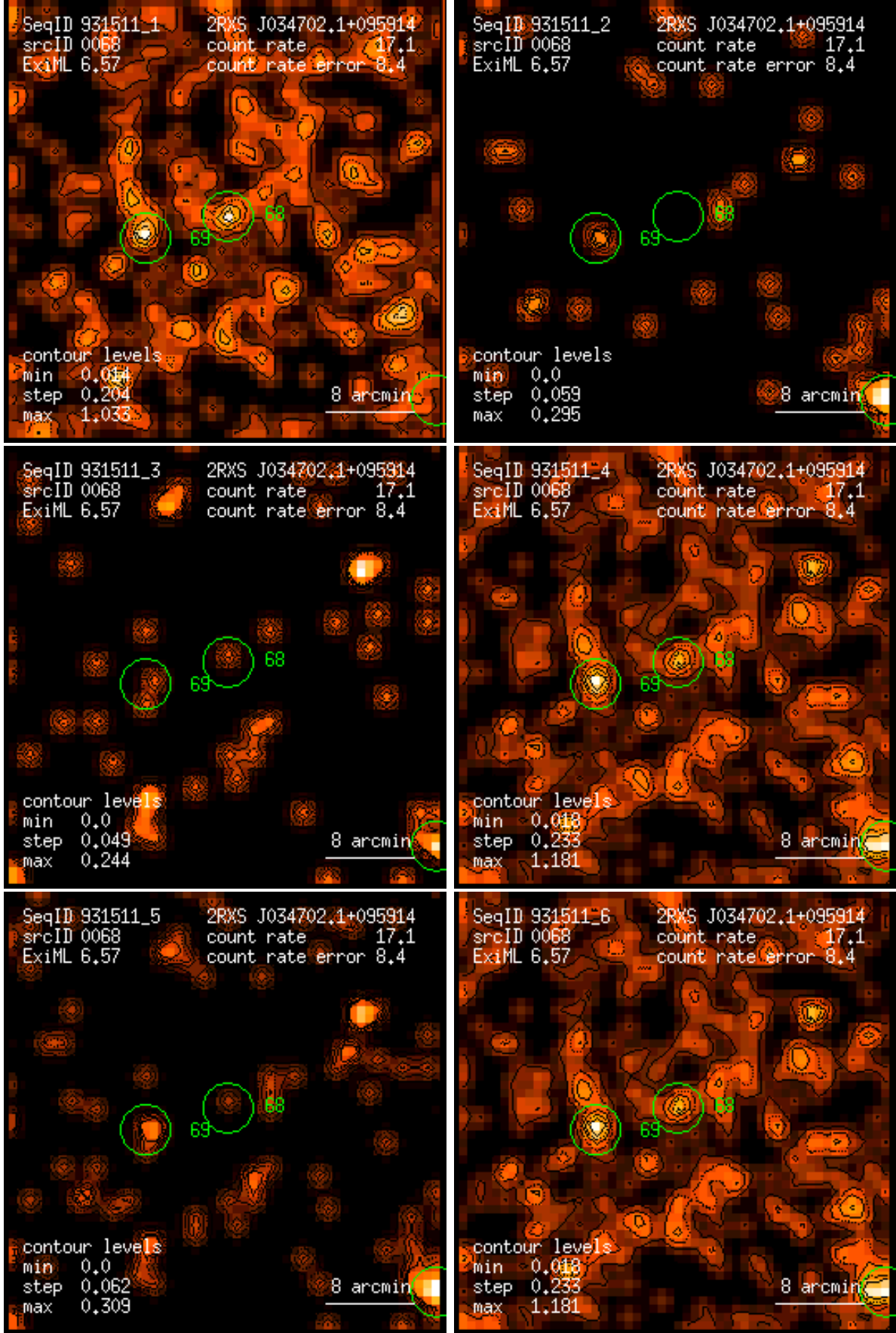
Figure 68: RASS 931511: detection 0068: band rate images, Gaussian filter: (1) PSPC channels 11 – 41, (2) 52 – 90, (3) 91 – 201, (4) 11 – 235, (5) 52 – 201, (6) 11 – 201. Broad band rates in counts/ks. Band rate contour levels in counts/ks/arcmin 2 .
