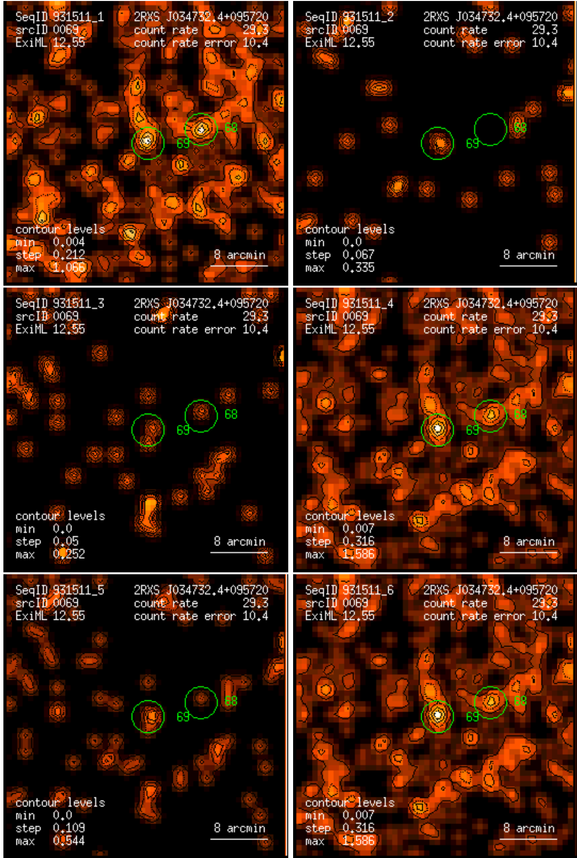
Figure 69: RASS 931511: detection 0069: band rate images, Gaussian filter: (1) PSPC channels 11 – 41, (2) 52 – 90, (3) 91 – 201, (4) 11 – 235, (5) 52 – 201, (6) 11 – 201. Broad band rates in counts/ks. Band rate contour levels in counts/ks/arcmin 2 .
